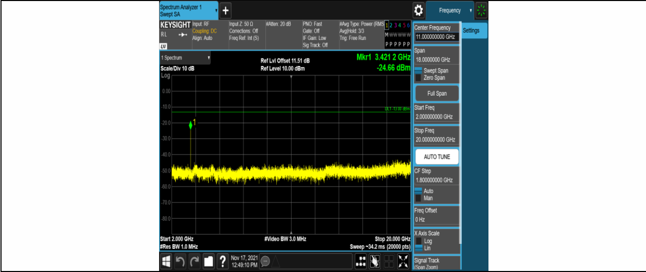
Band4-5MHz-QPSK-19975-1RB#0-Range3:2000~20000MHz
