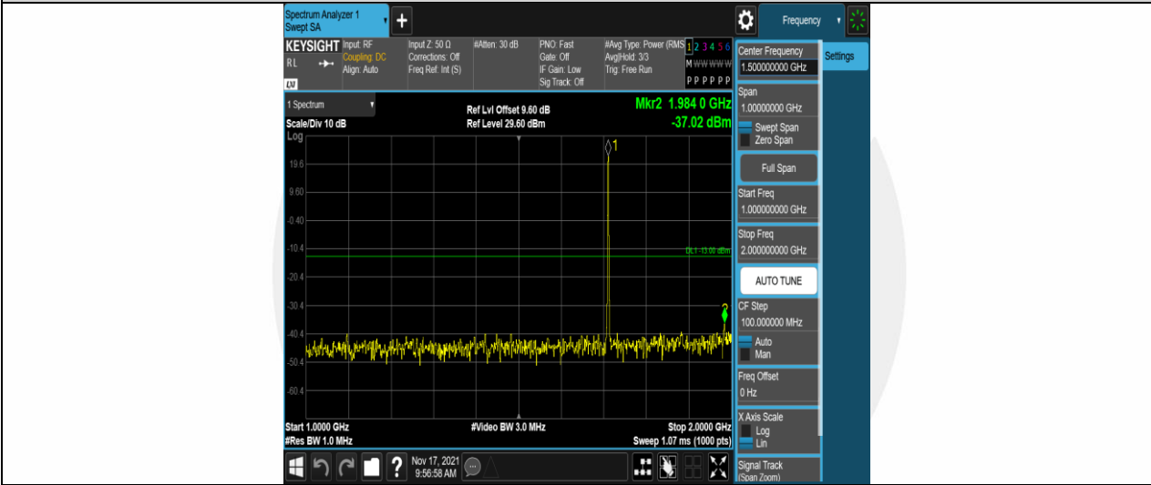
Band4-1.4MHz-16QAM-19957-1RB#0-Range2:1000~2000MHz
