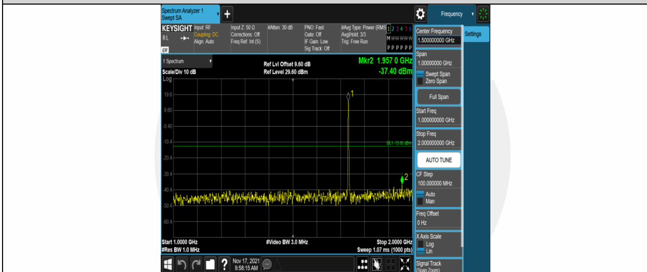
Band4-1.4MHz-16QAM-20175-1RB#0-Range2:1000~2000MHz
