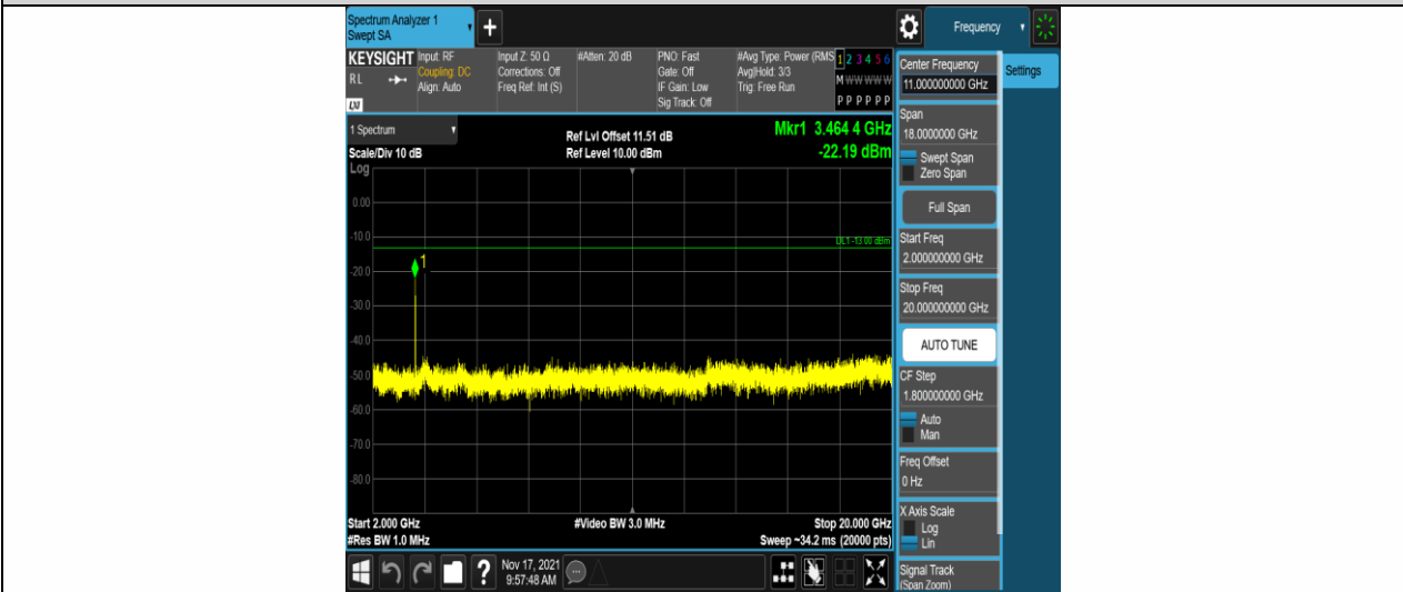
Band4-1.4MHz-QPSK-20175-1RB#0-Range3:2000~20000MHz
