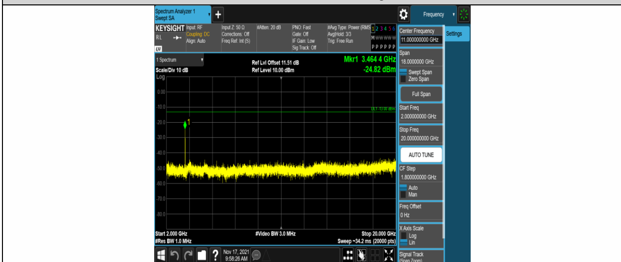
Band4-1.4MHz-16QAM-20175-1RB#0-Range3:2000~20000MHz
