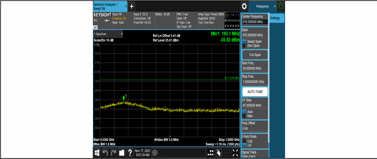
Band4-1.4MHz-QPSK-20175-1RB#0-Range1:30~1000MHz
