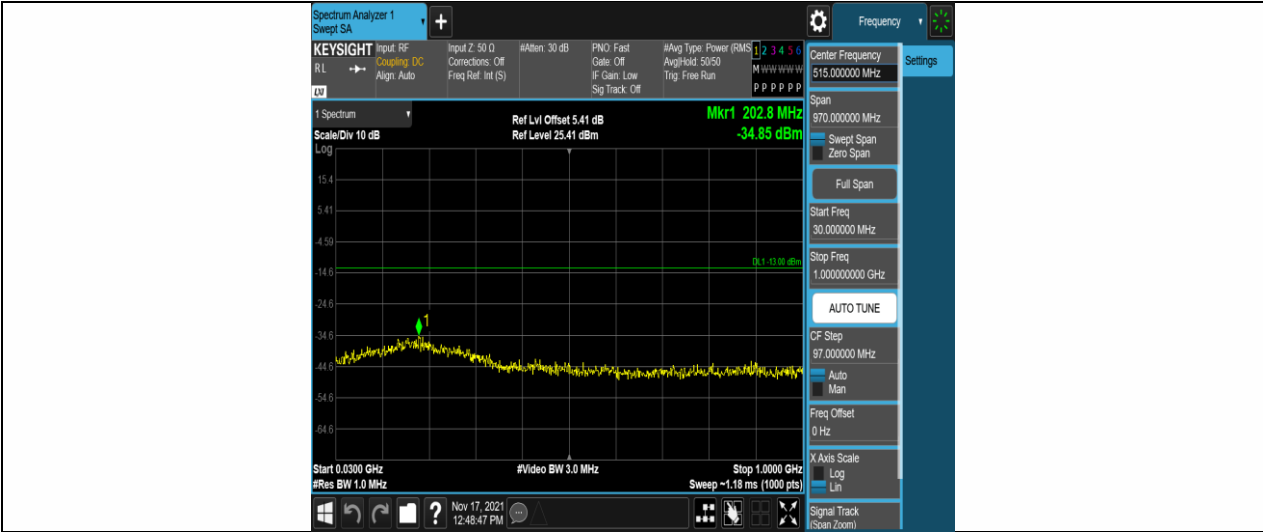
Band4-5MHz-QPSK-19975-1RB#0-Range1:30~1000MHz
