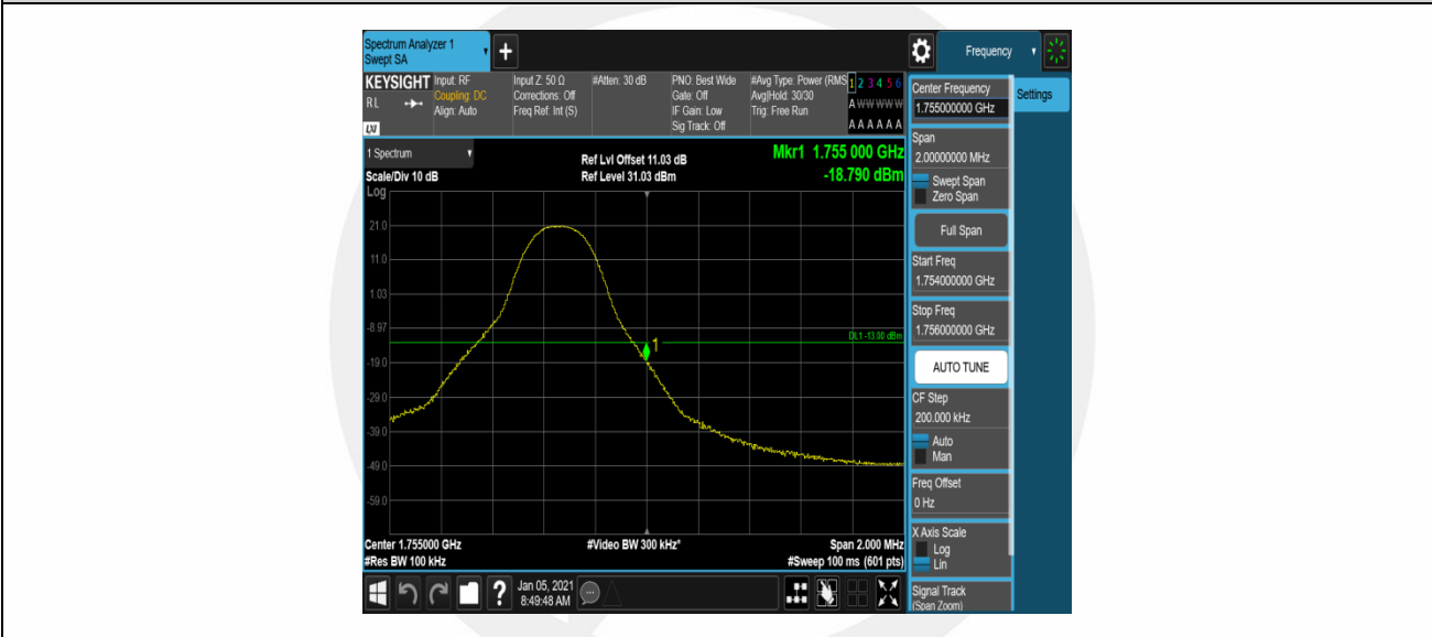
Band4-5MHz-QPSK-20375-1RB#24
