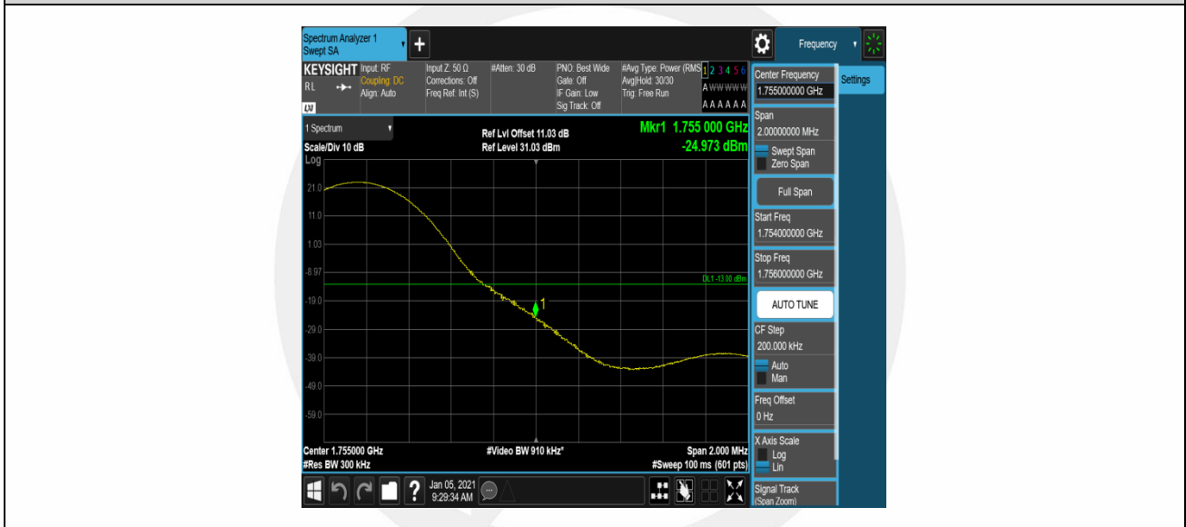
Band4-15MHz-QPSK-20325-1RB#74
