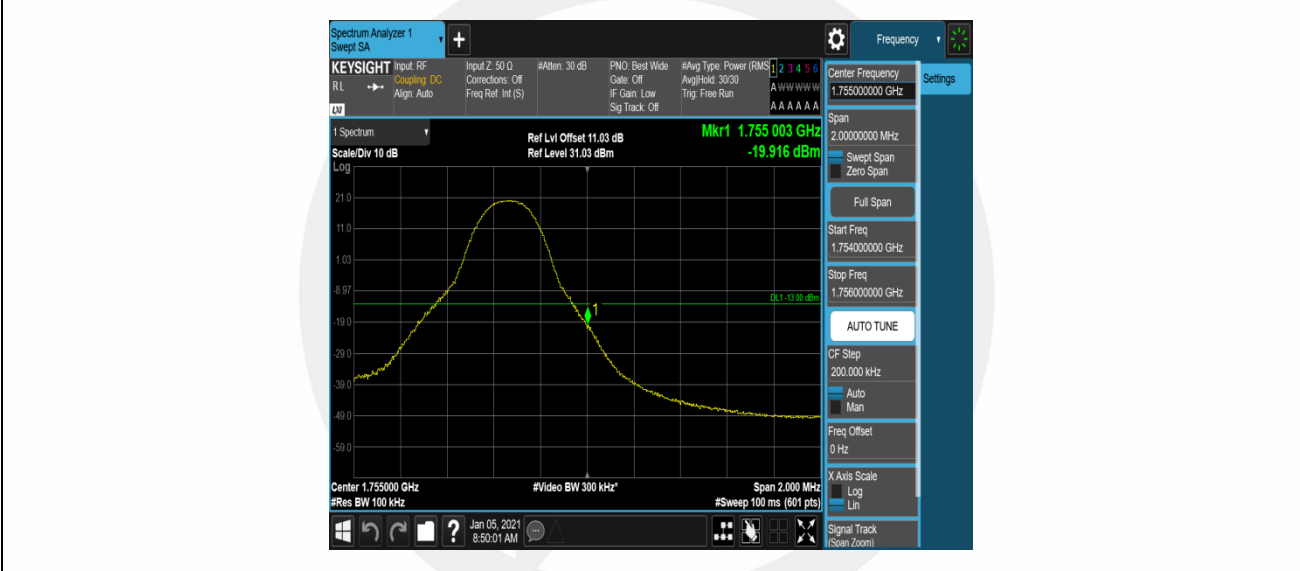
Band4-5MHz-16QAM-20375-1RB#24
