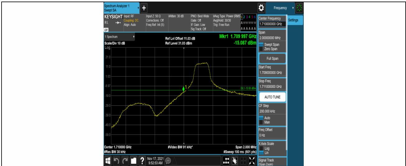
Band4-1.4MHz-16QAM-19957-1RB#0
