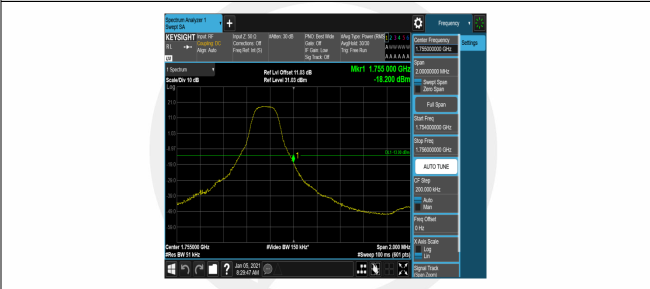
Band4-3MHz-QPSK-20385-1RB#14
