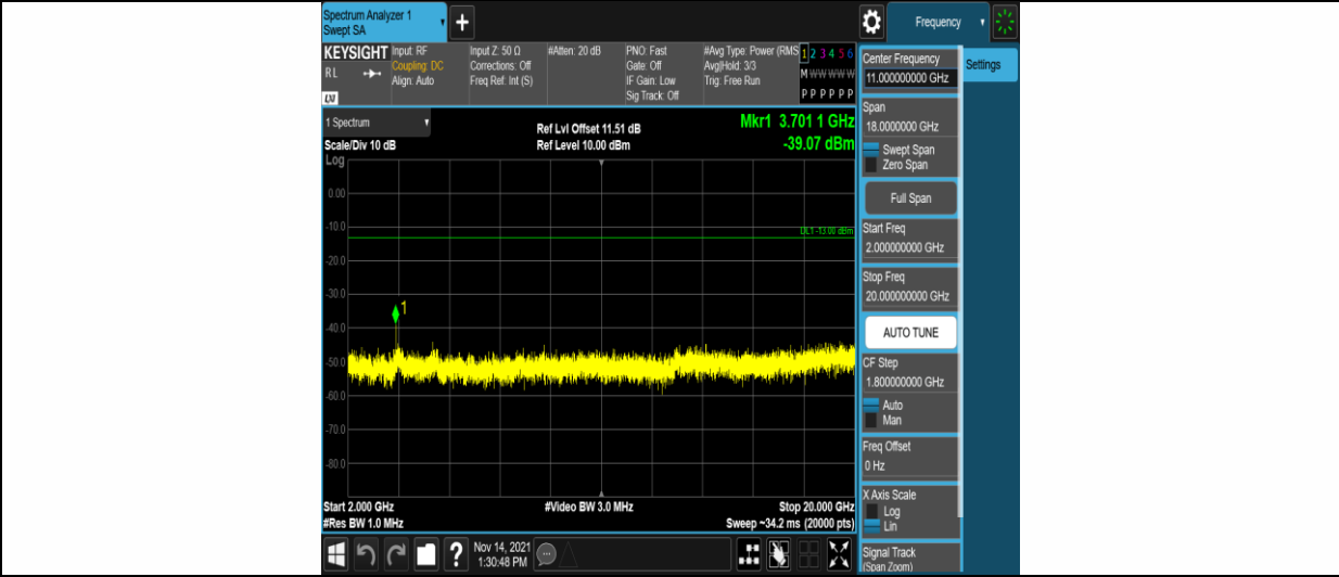
Band2-1.4MHz-16QAM-18607-1RB#0-Range3:2000~20000MHz
