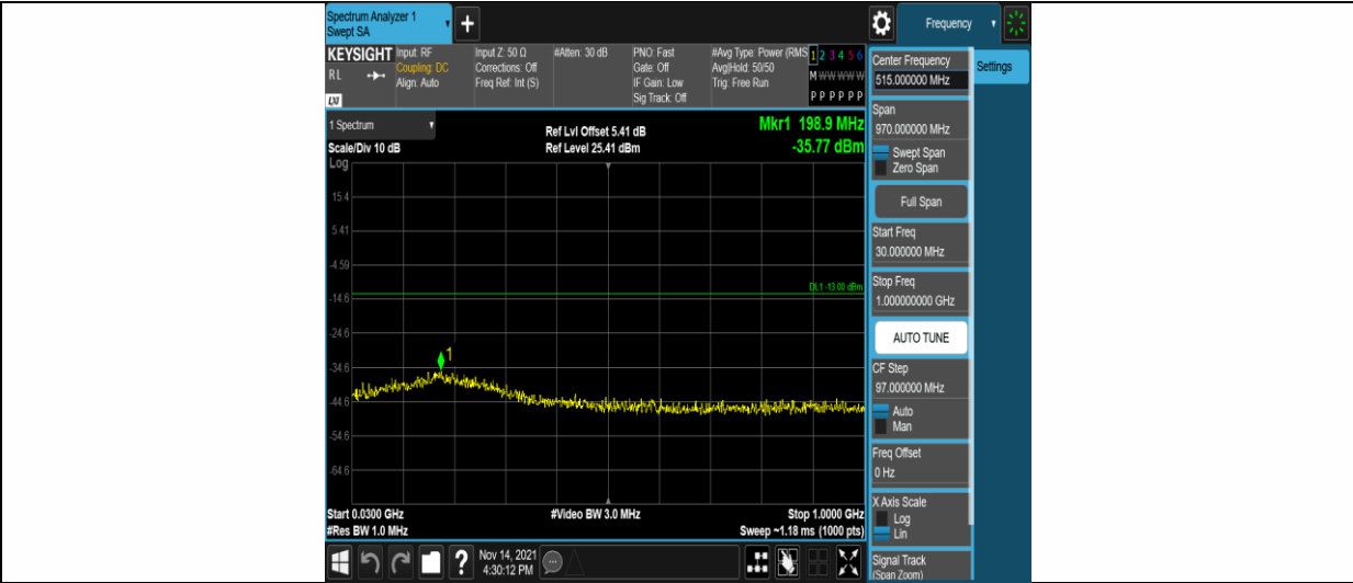
Band2-3MHz-QPSK-18900-1RB#0-Range1:30~1000MHz
