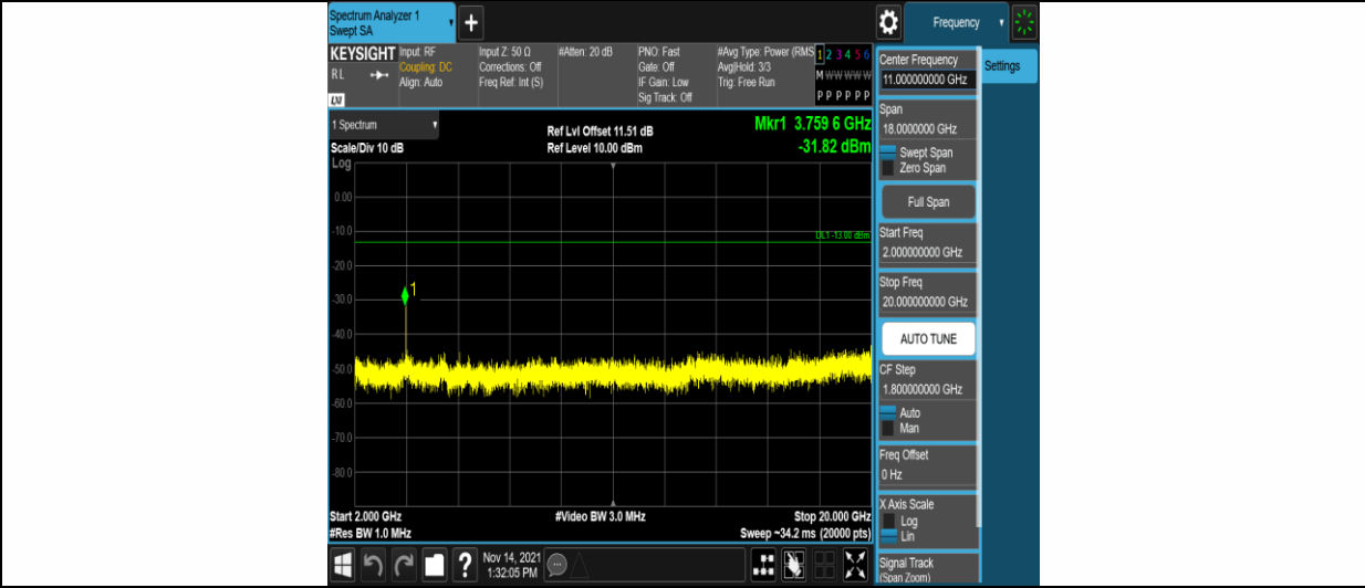
Band2-1.4MHz-16QAM-18900-1RB#0-Range3:2000~20000MHz
