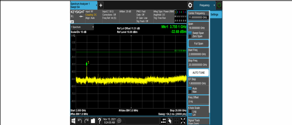
Band2-5MHz-QPSK-18900-1RB#0-Range3:2000~20000MHz
