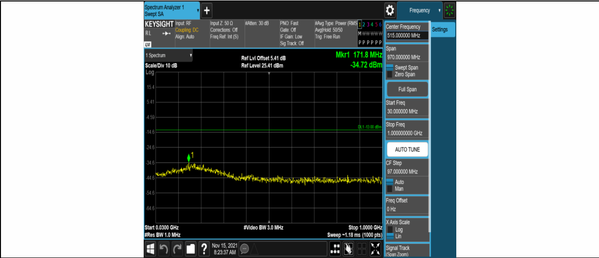
Band2-5MHz-QPSK-18900-1RB#0-Range1:30~1000MHz
