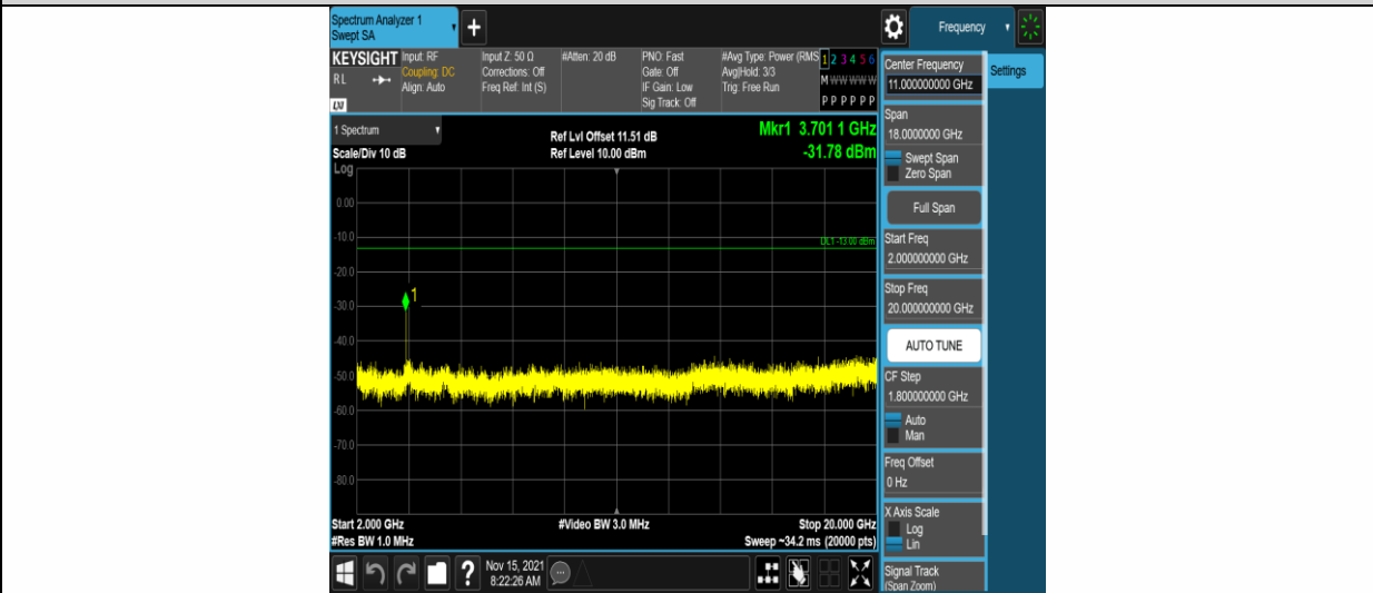
Band2-5MHz-QPSK-18625-1RB#0-Range3:2000~20000MHz
