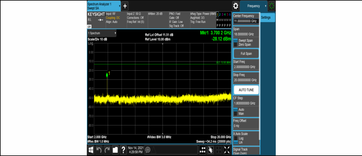
Band2-3MHz-16QAM-18615-1RB#0-Range3:2000~20000MHz
