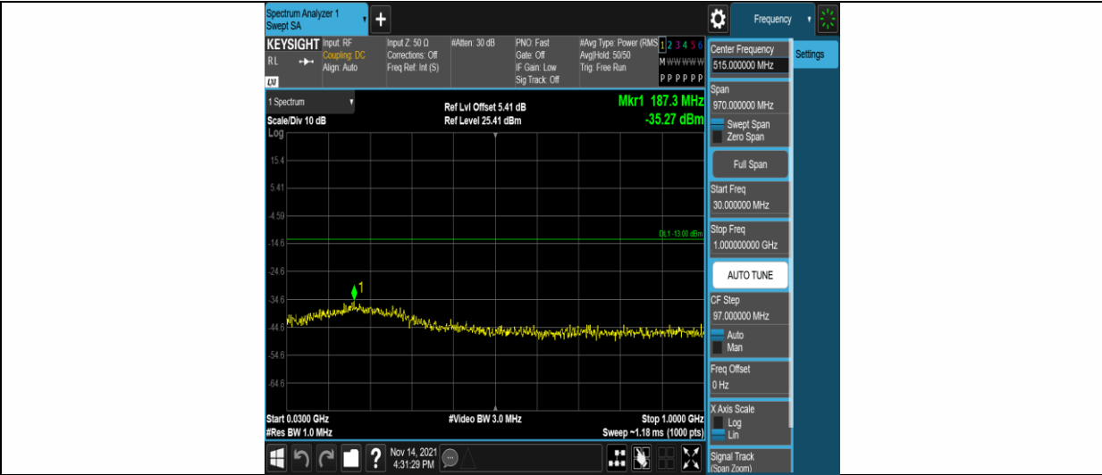
Band2-3MHz-QPSK-19185-1RB#0-Range1:30~1000MHz
