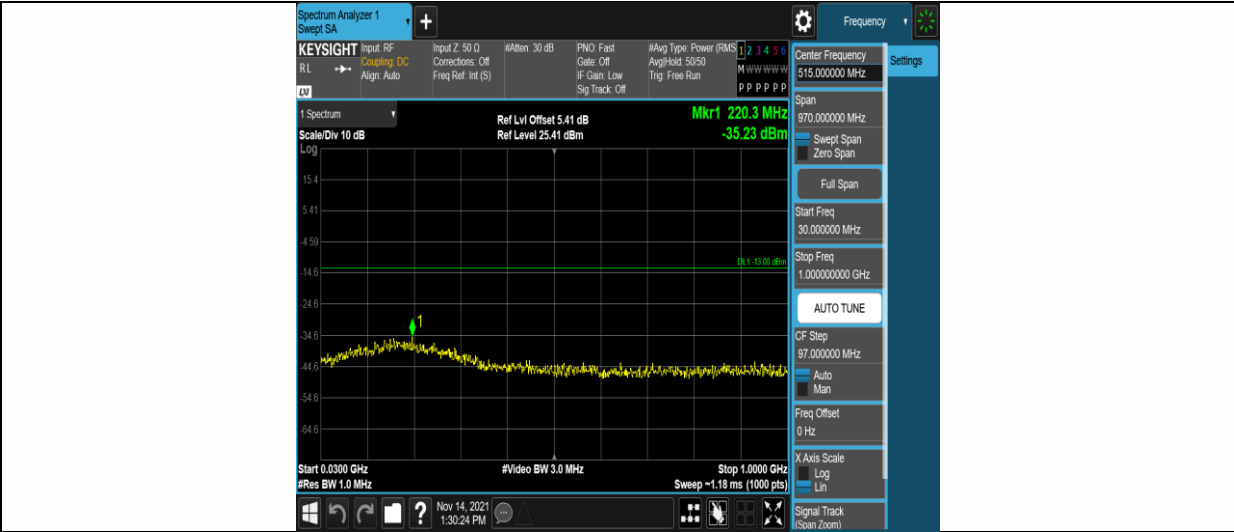
Band2-1.4MHz-16QAM-18607-1RB#0-Range1:30~1000MHz
