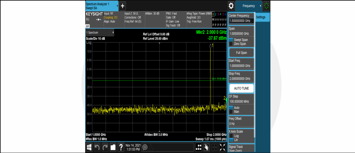
Band2-1.4MHz-16QAM-18900-1RB#0-Range2:1000~2000MHz
