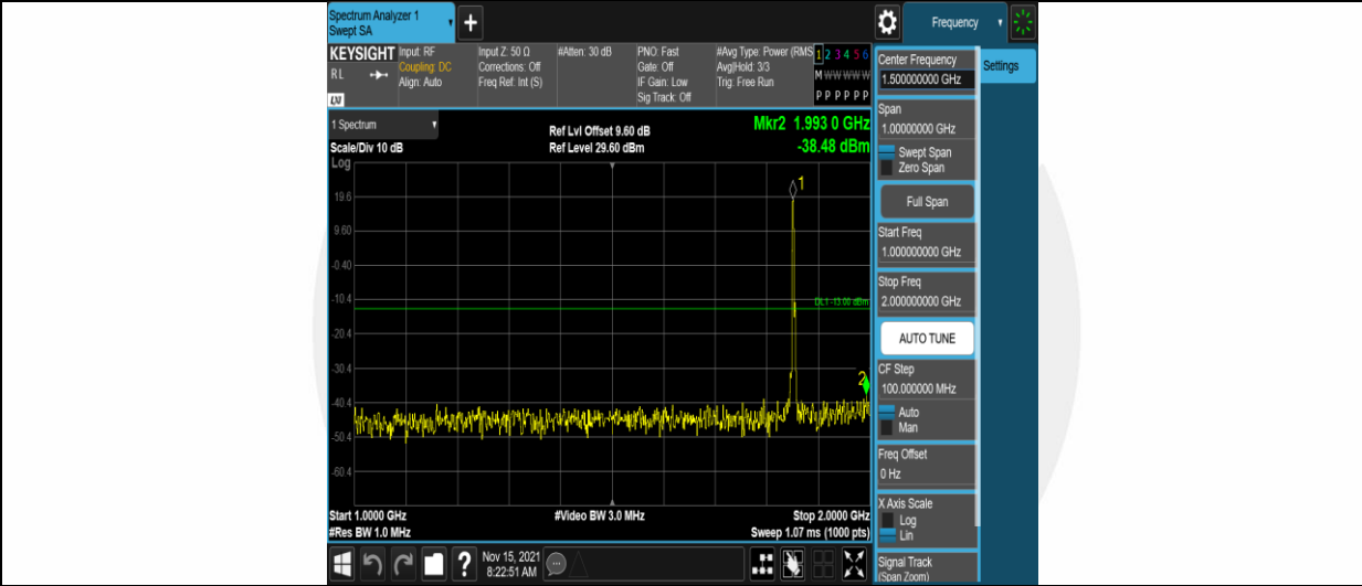
Band2-5MHz-16QAM-18625-1RB#0-Range2:1000~2000MHz
