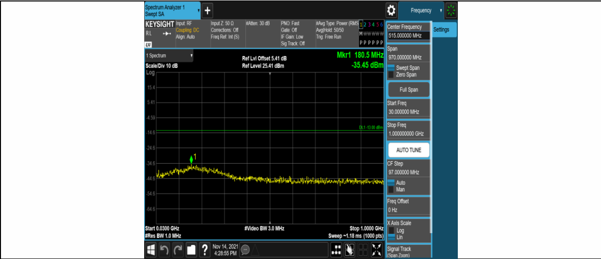
Band2-3MHz-QPSK-18615-1RB#0-Range1:30~1000MHz
