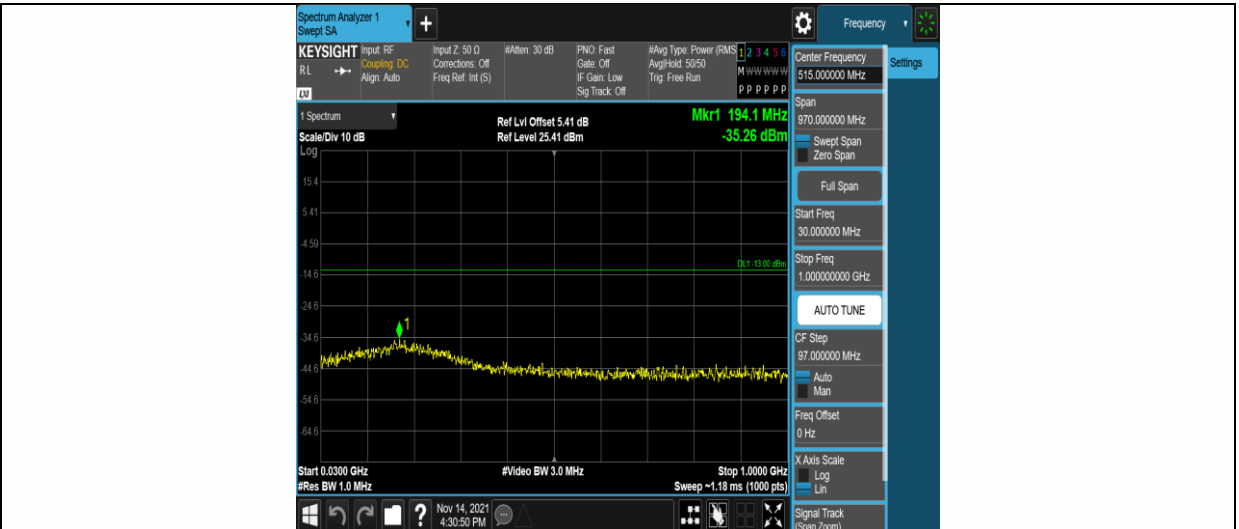
Band2-3MHz-16QAM-18900-1RB#0-Range1:30~1000MHz
