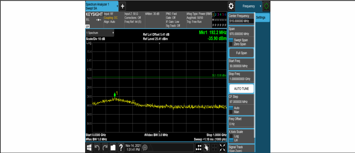
Band2-1.4MHz-16QAM-18900-1RB#0-Range1:30~1000MHz
