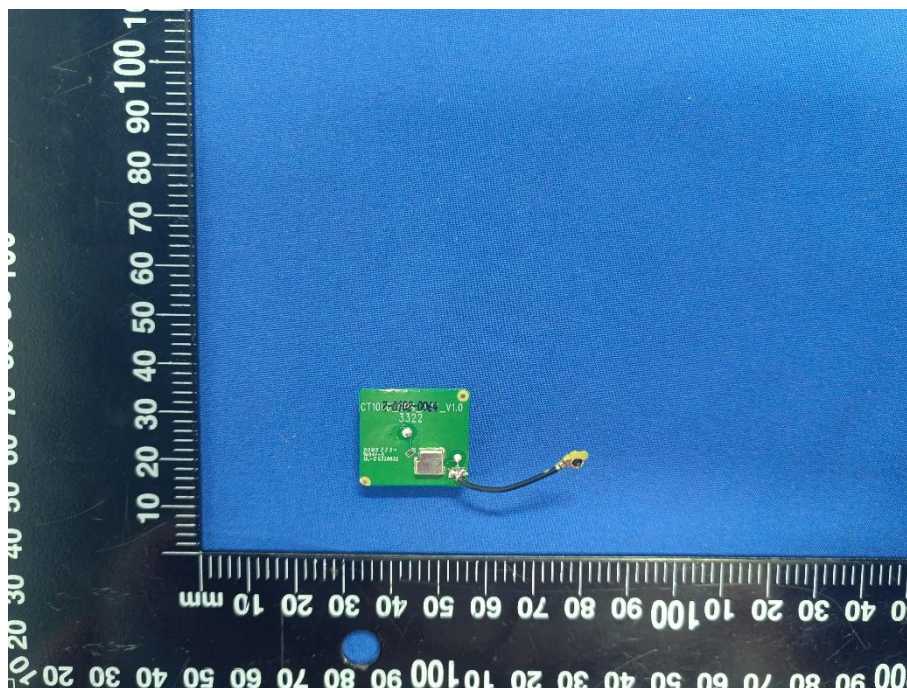
SUB BOARD TOP VIEW 2 (WITH SHIELDING)
