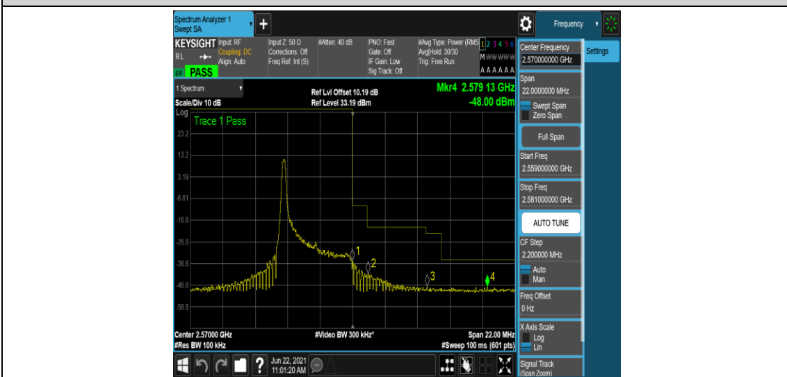
Band7-5MHz-16QAM-21425-1RB#24
