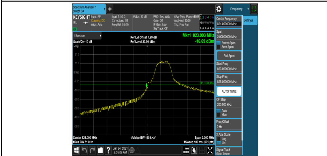
Band5-3MHz-16QAM-20415-1RB#14
