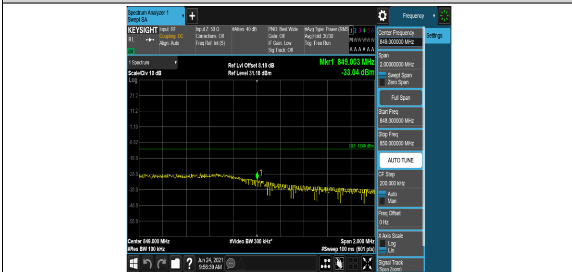
Band5-5MHz-16QAM-20625-1RB#24
