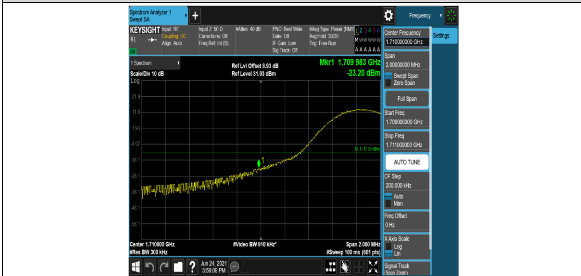
Band4-15MHz-16QAM-20025-1RB#74
