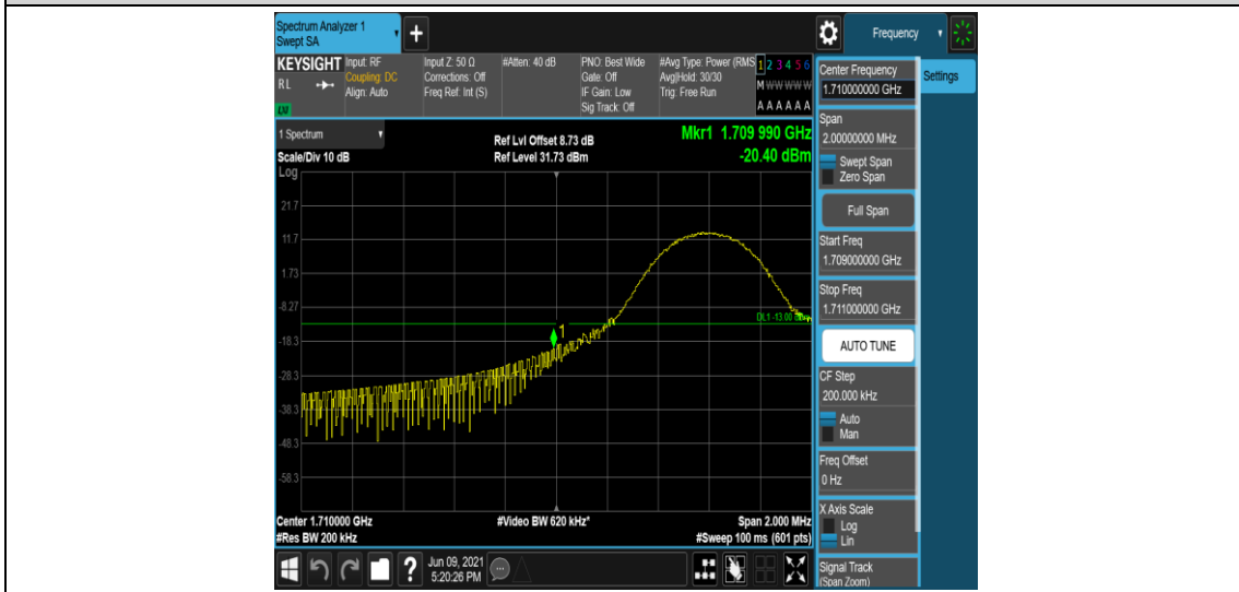
Band4-10MHz-16QAM-20000-1RB#49
