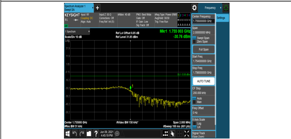
Band4-3MHz-16QAM-20385-1RB#14
