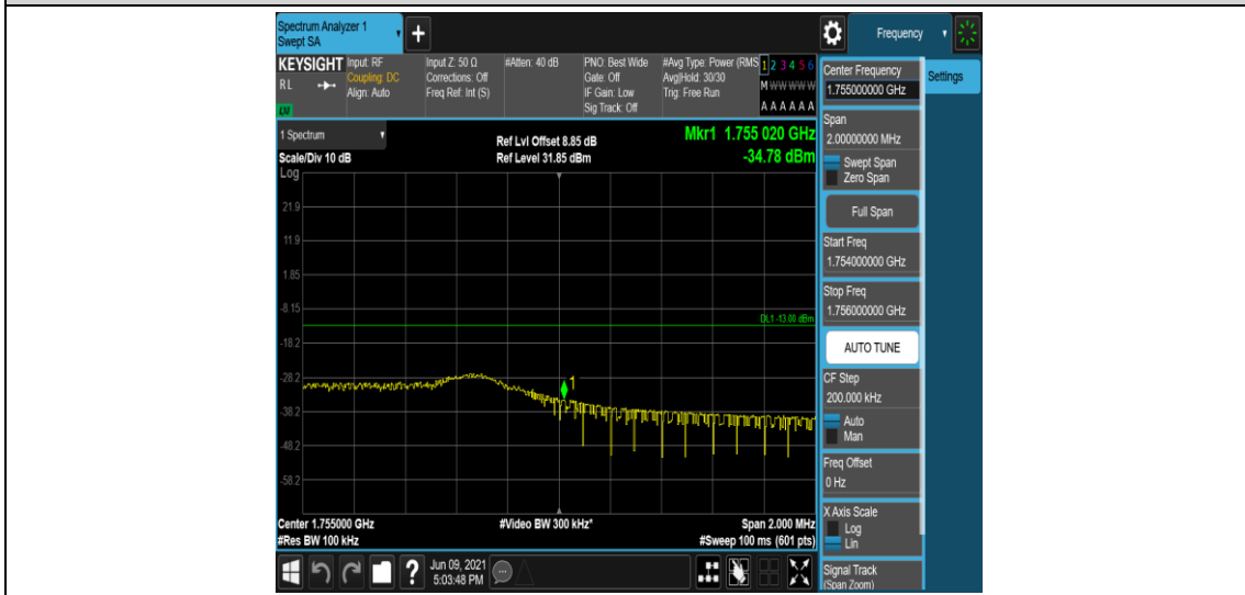
Band4-5MHz-QPSK-20375-1RB#24
