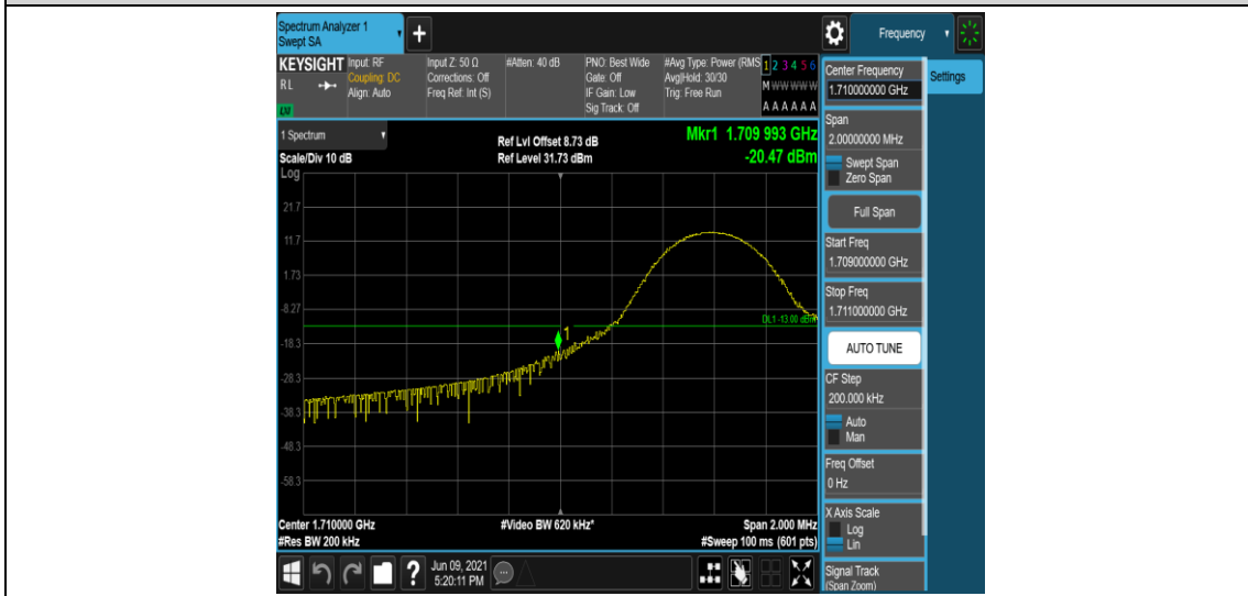
Band4-10MHz-QPSK-20000-1RB#49
