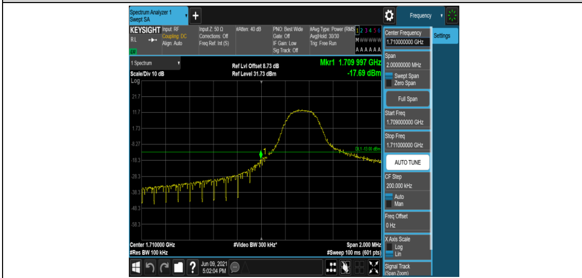
Band4-5MHz-QPSK-19975-1RB#24
