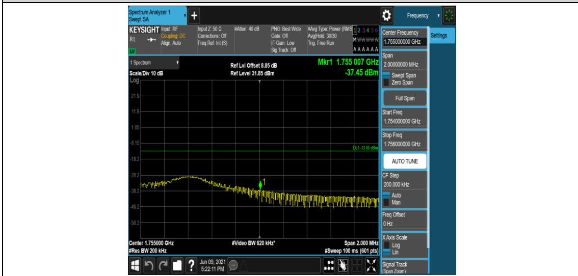
Band4-10MHz-16QAM-20350-1RB#49
