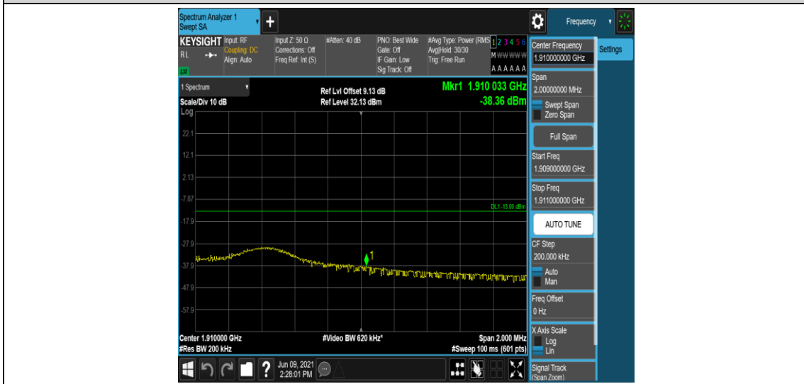
Band2-10MHz-QPSK-19150-1RB#49
