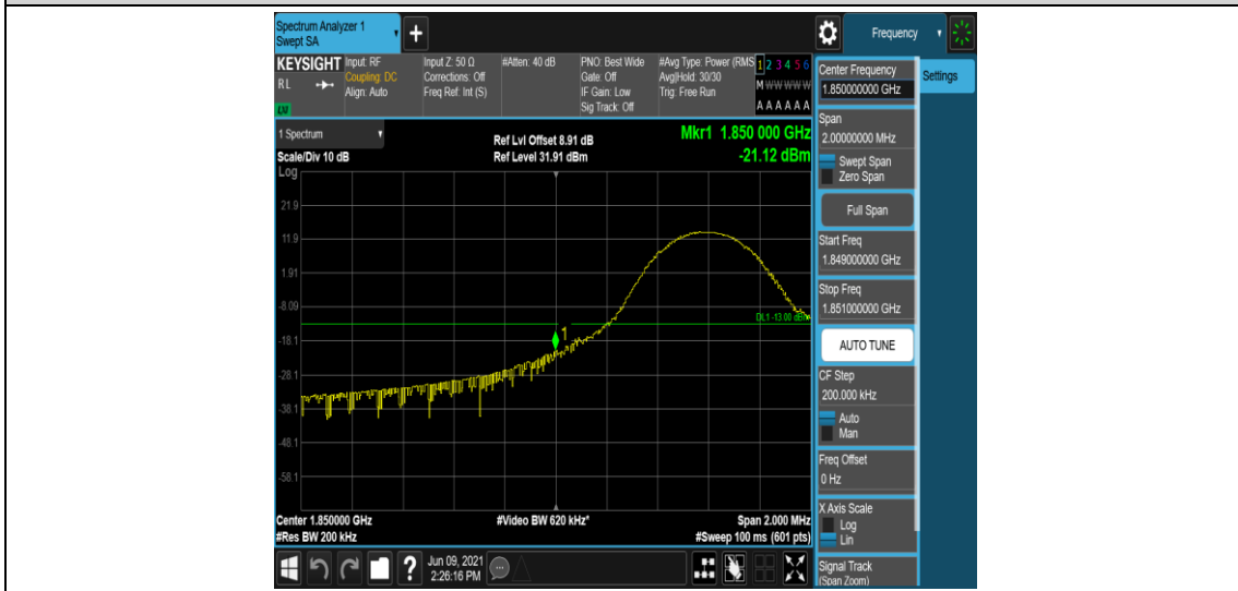
Band2-10MHz-QPSK-18650-1RB#49
