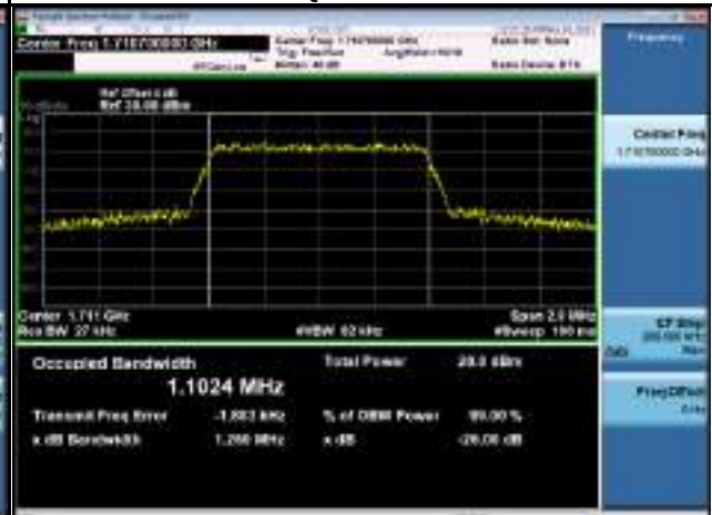
16QAM-20393
