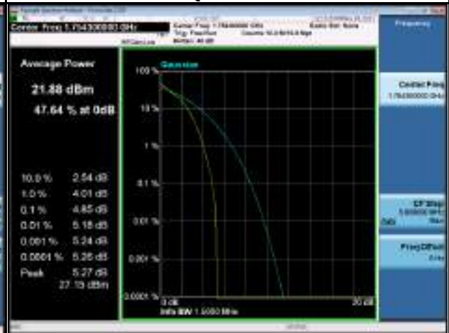
16QAM-20393
