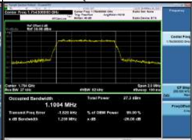
16QAM-20393
