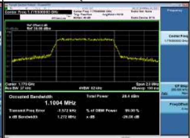
16QAM-132665
