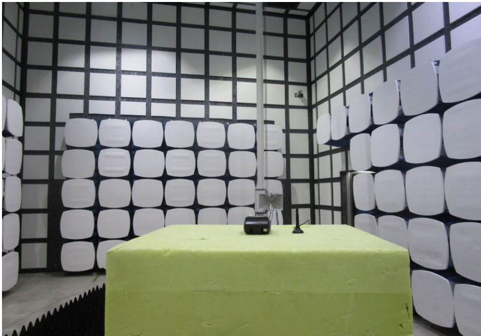
Spurious emissions at antenna terminals (Above 1GHz)
