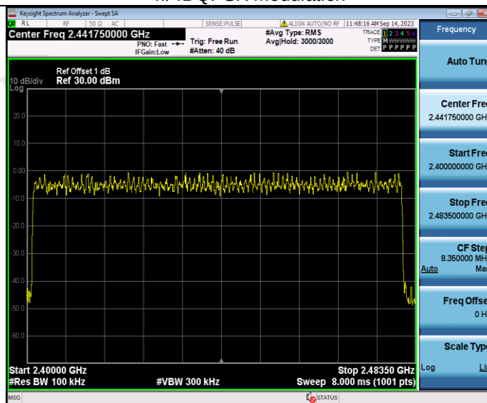
8DPSK Modulation
