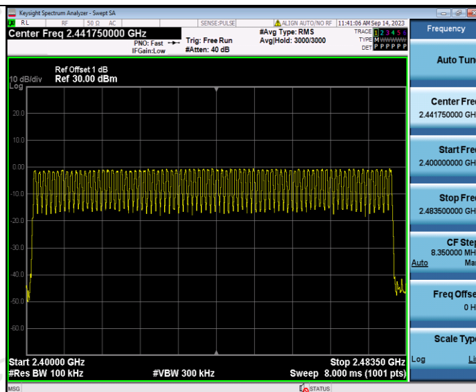
GFSK Modulation
