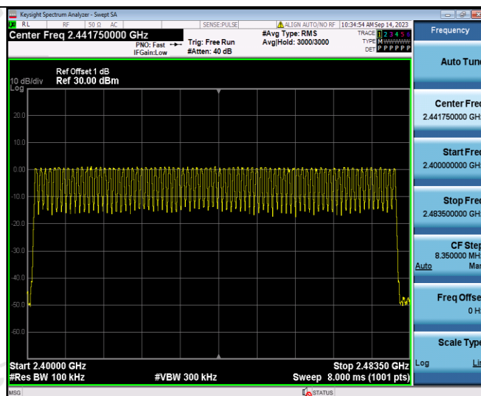
GFSK Modulation
