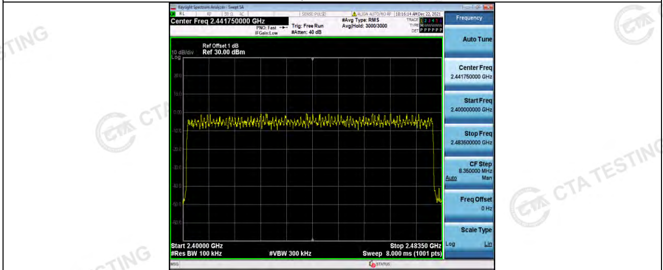
8DPSK Modulation
