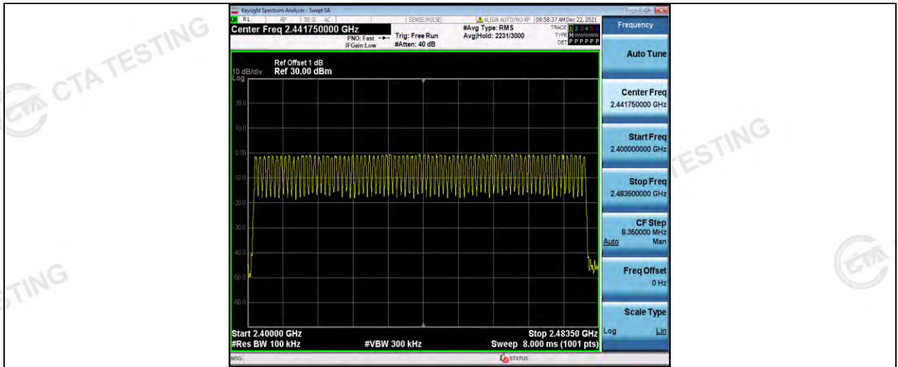
GFSK Modulation
