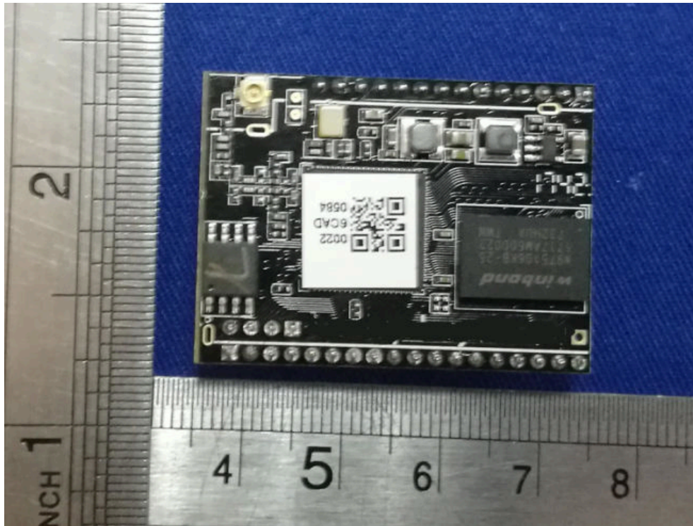
EUT – Antenna View 5
