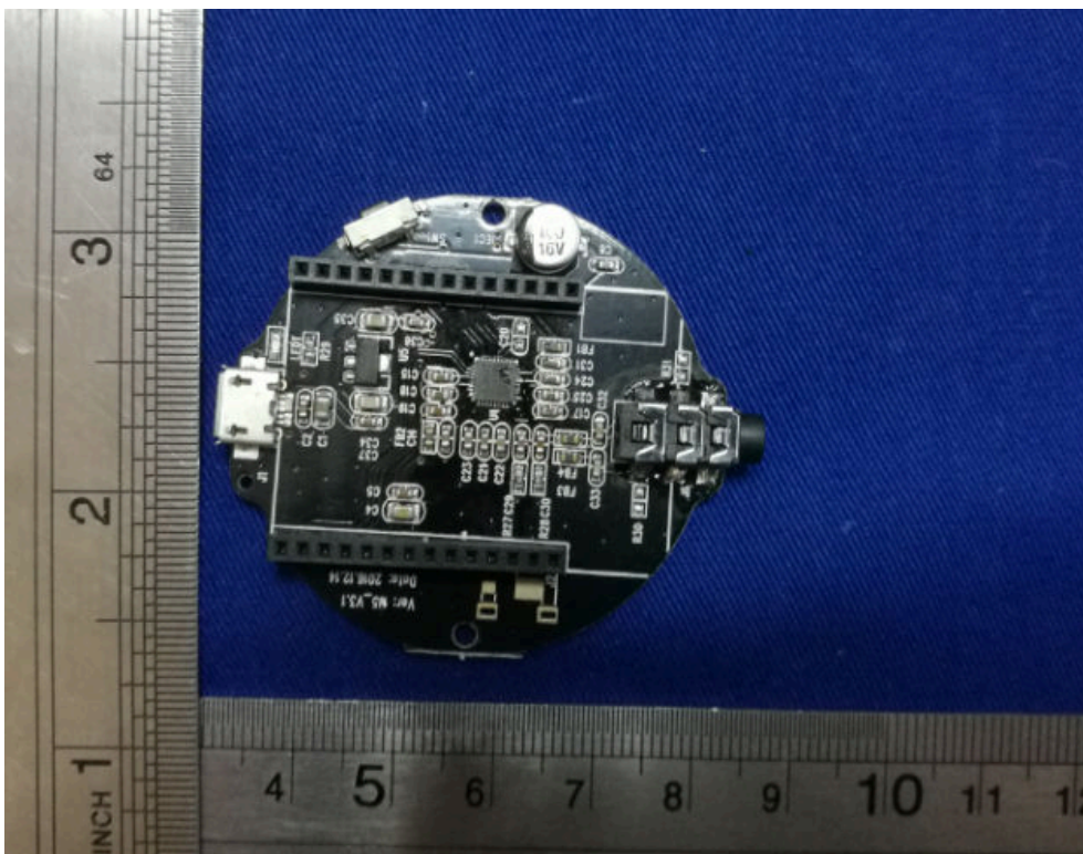
EUT - PCB View 1
