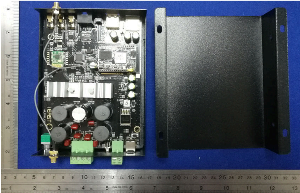
EUT - PCB View 1
