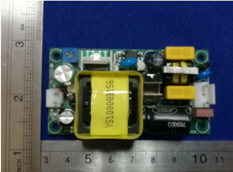
EUT – PCB View 7
