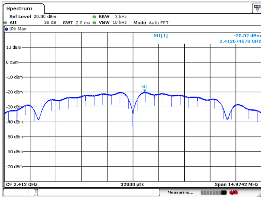
802.11b-Low Channel
