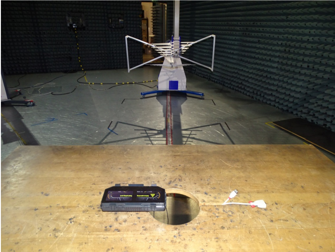
Photo 1: Test setup for radiated measurements (stand alone, EUT supplied by a battery) 30 MHz - 1 GHz
