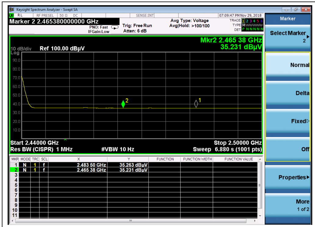
(2440MHz, AVG)
