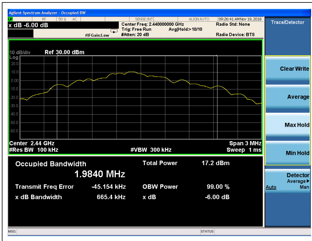
(2440 MHz)
