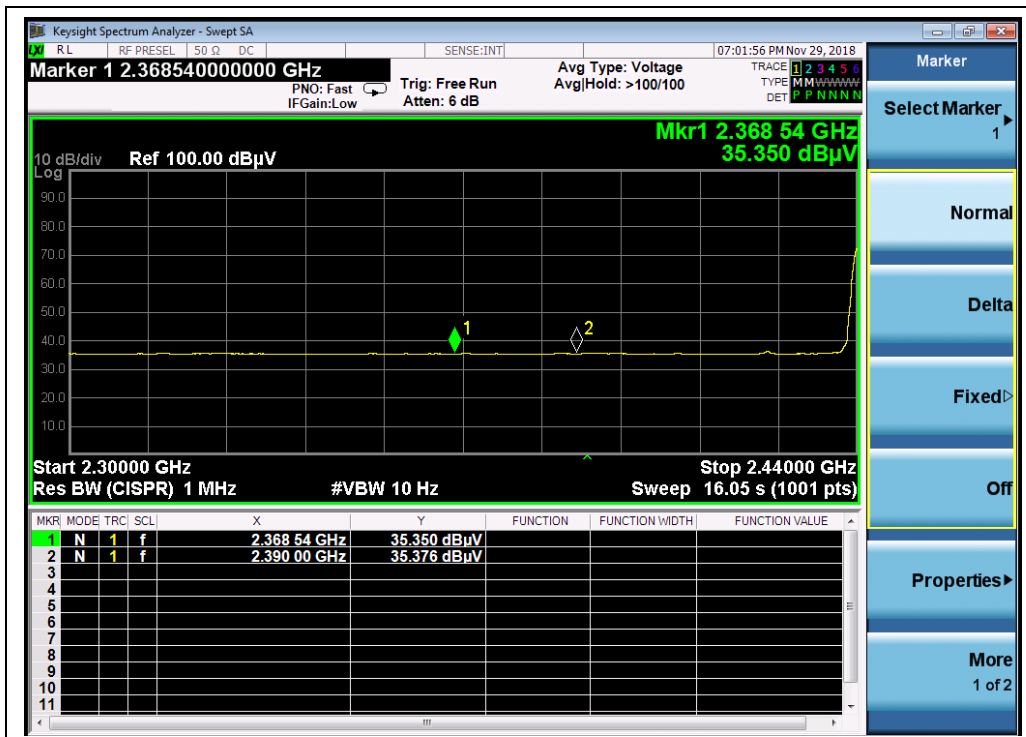
(2440MHz, AVG)
