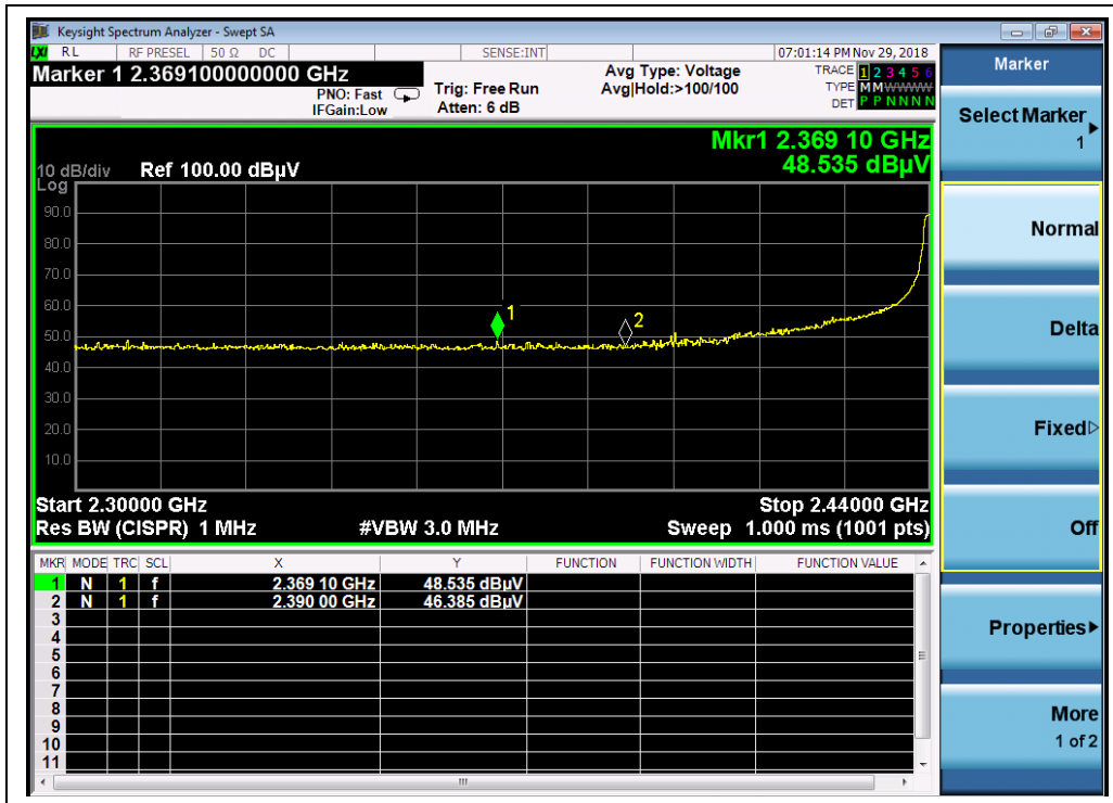
(2440MHz, PEAK)
