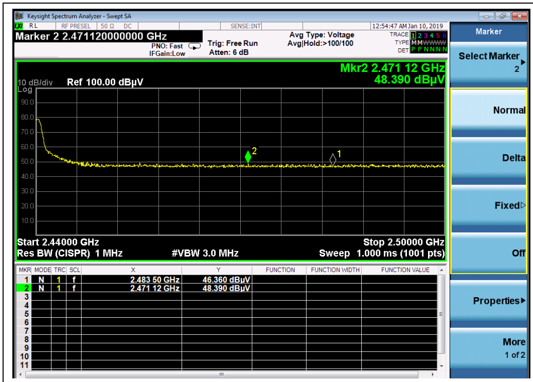
(2440MHz, PEAK)
