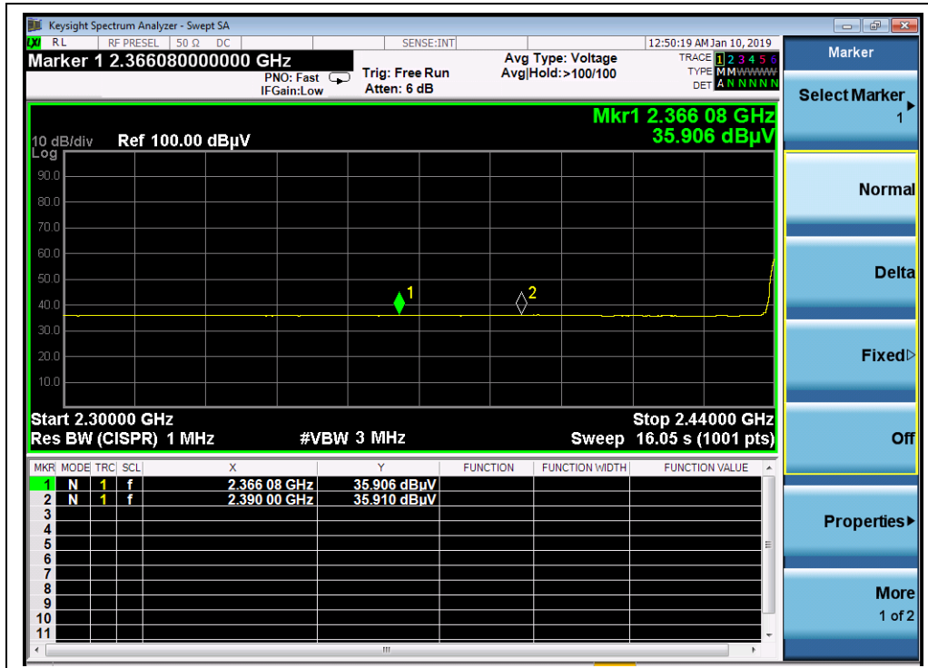
(2440MHz, AVG)
