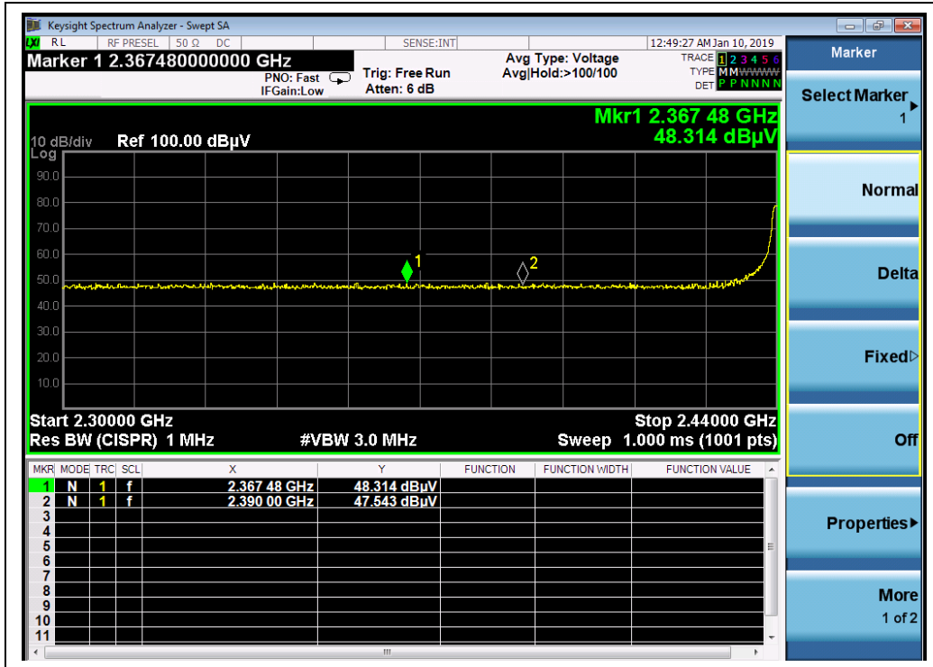
(2440MHz, PEAK)
