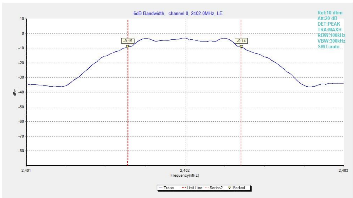
Fig.7 6dB Bandwidth (Ch 0)
