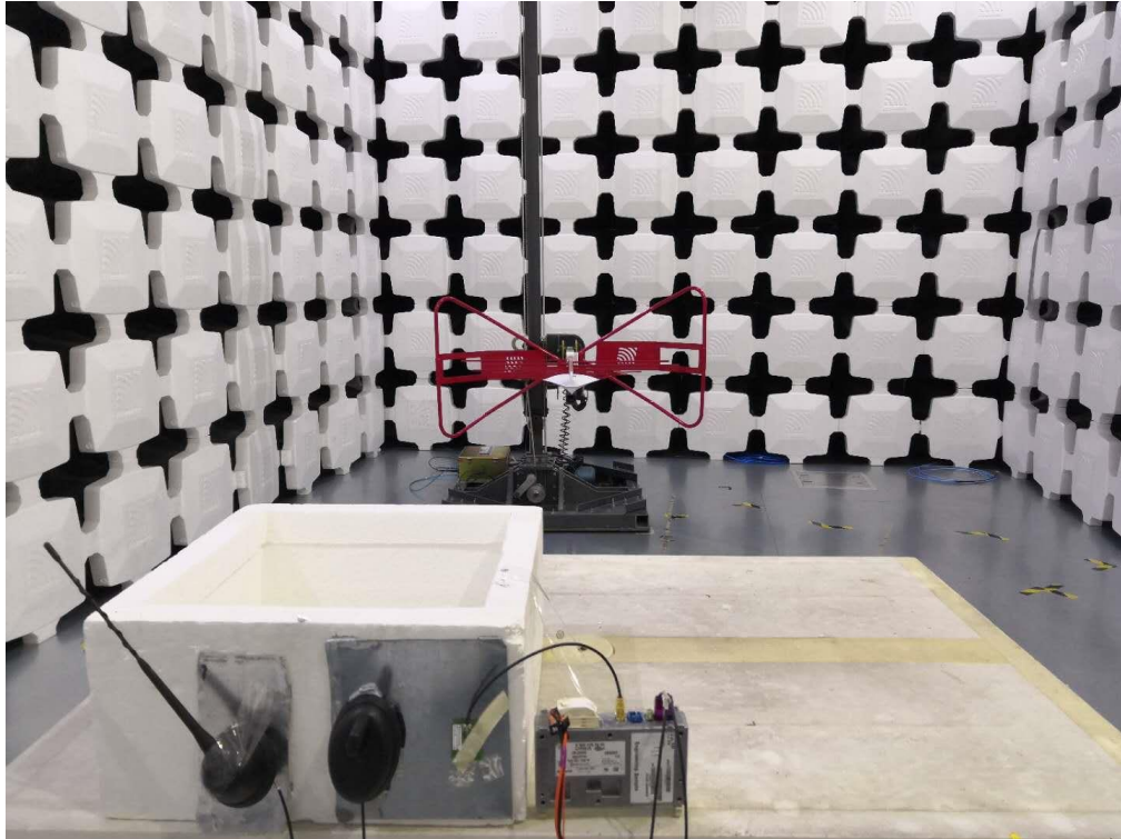
4. Radiated Emissions (Part 15C) (30MHz-1GHz,EUT-V)
