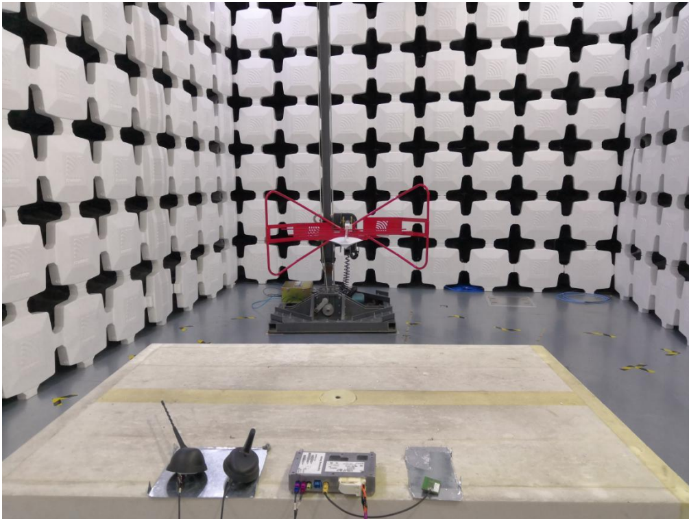
3. Radiated Emissions (Part 15C) (30MHz-1GHz,EUT-H)
