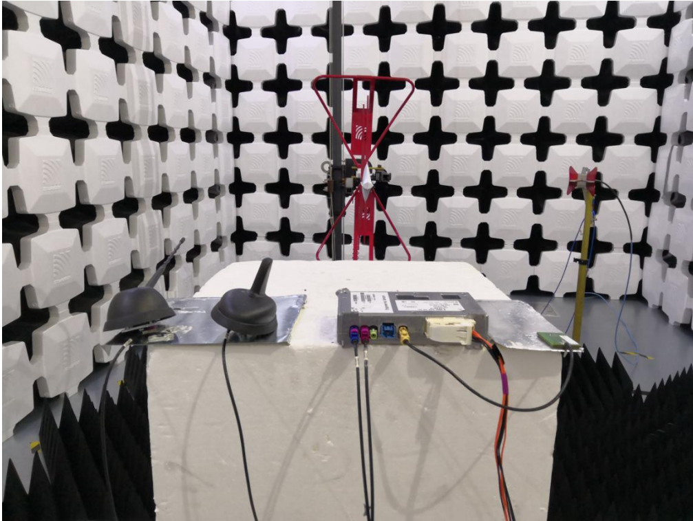
5. Radiated Emissions (Part 15C 1-18GHz,EUT-H)
