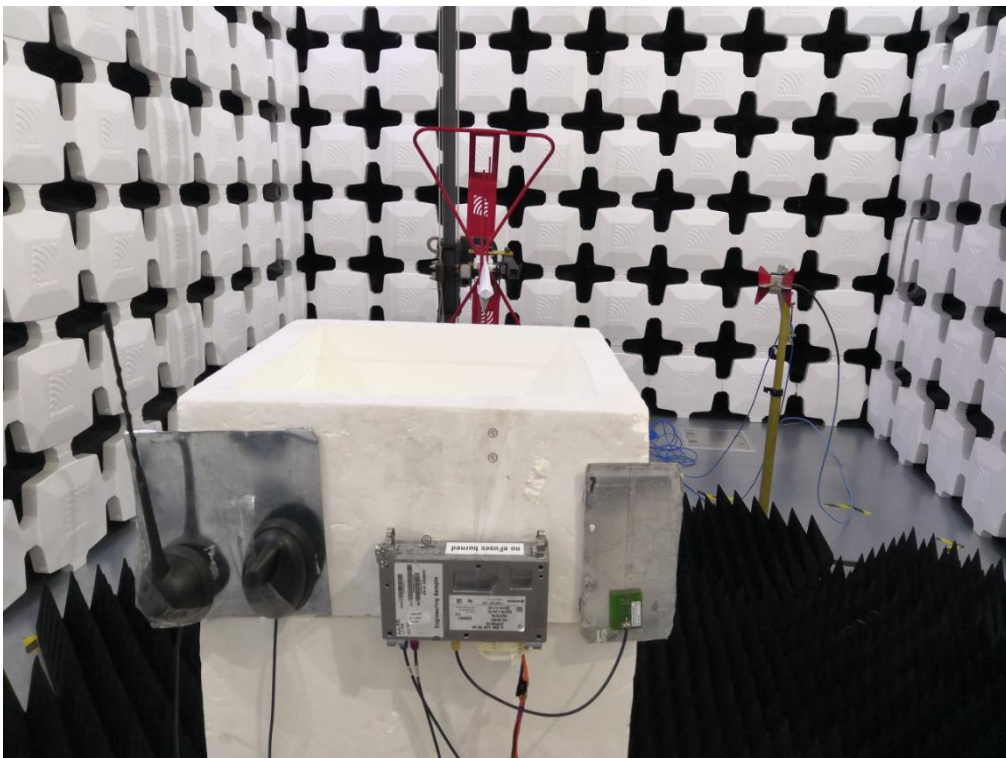
6. Radiated Emissions (Part 15C 1-18GHz,EUT-V)
