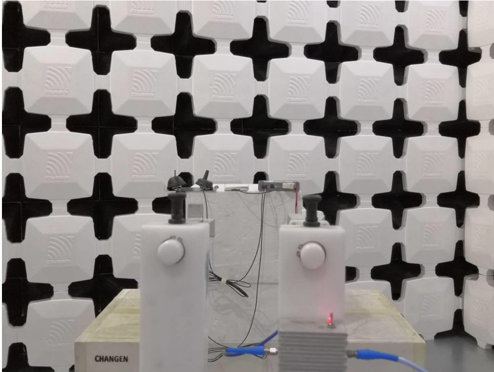
7. Radiated Emissions (Part 15C) (18GHz-26.5GHz,EUT-H)
