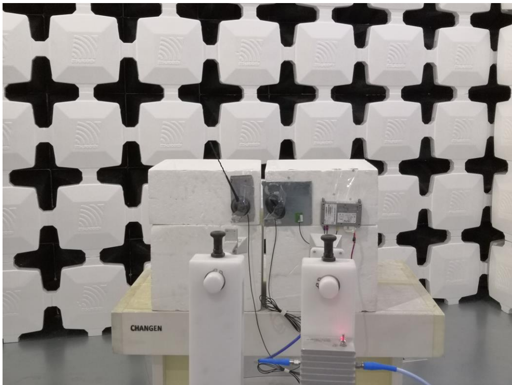
8. Radiated Emissions (Part 15C) (18GHz-26.5GHz,EUT-V)
