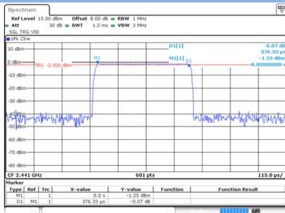
GFSK DH1
