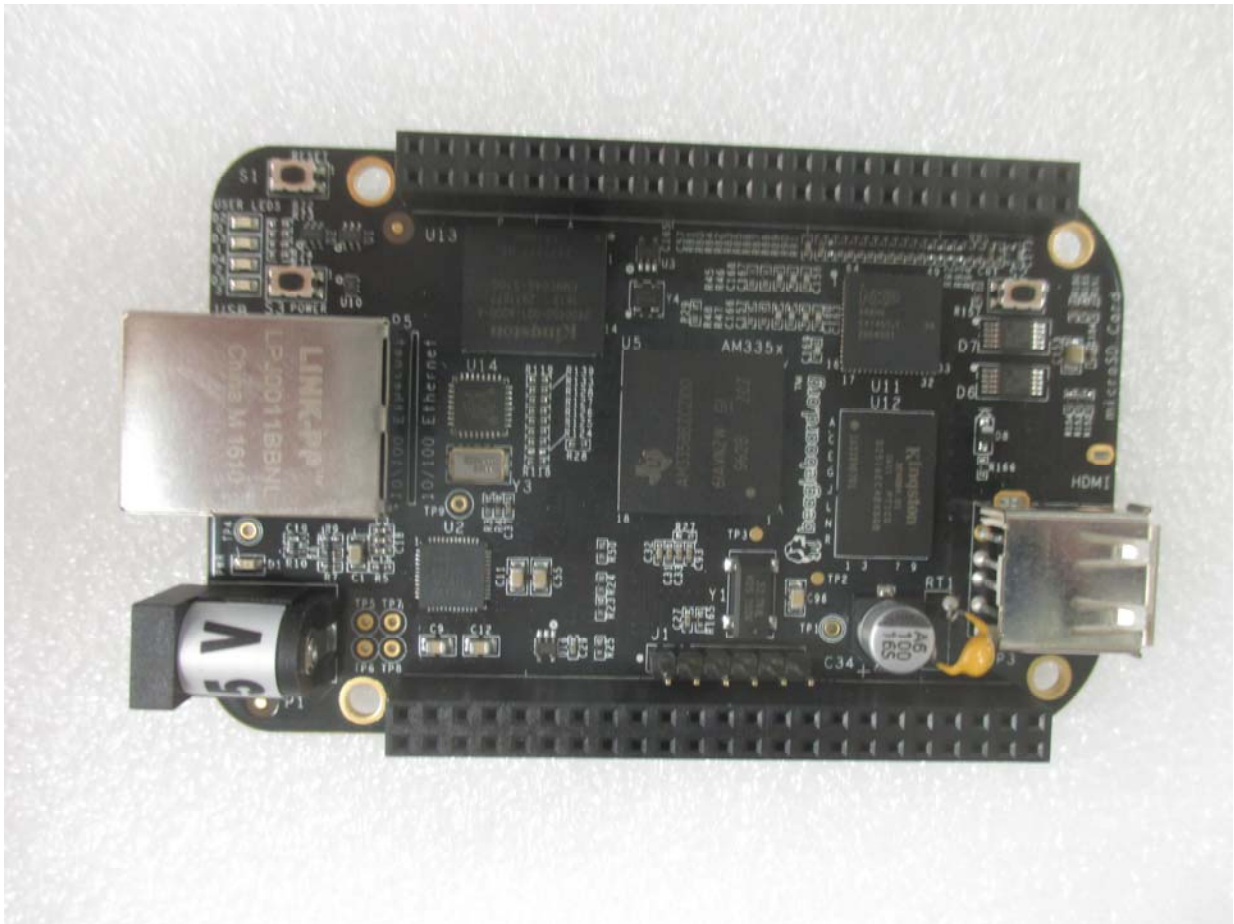
8.9 UHF Daughter Board Components Side View
