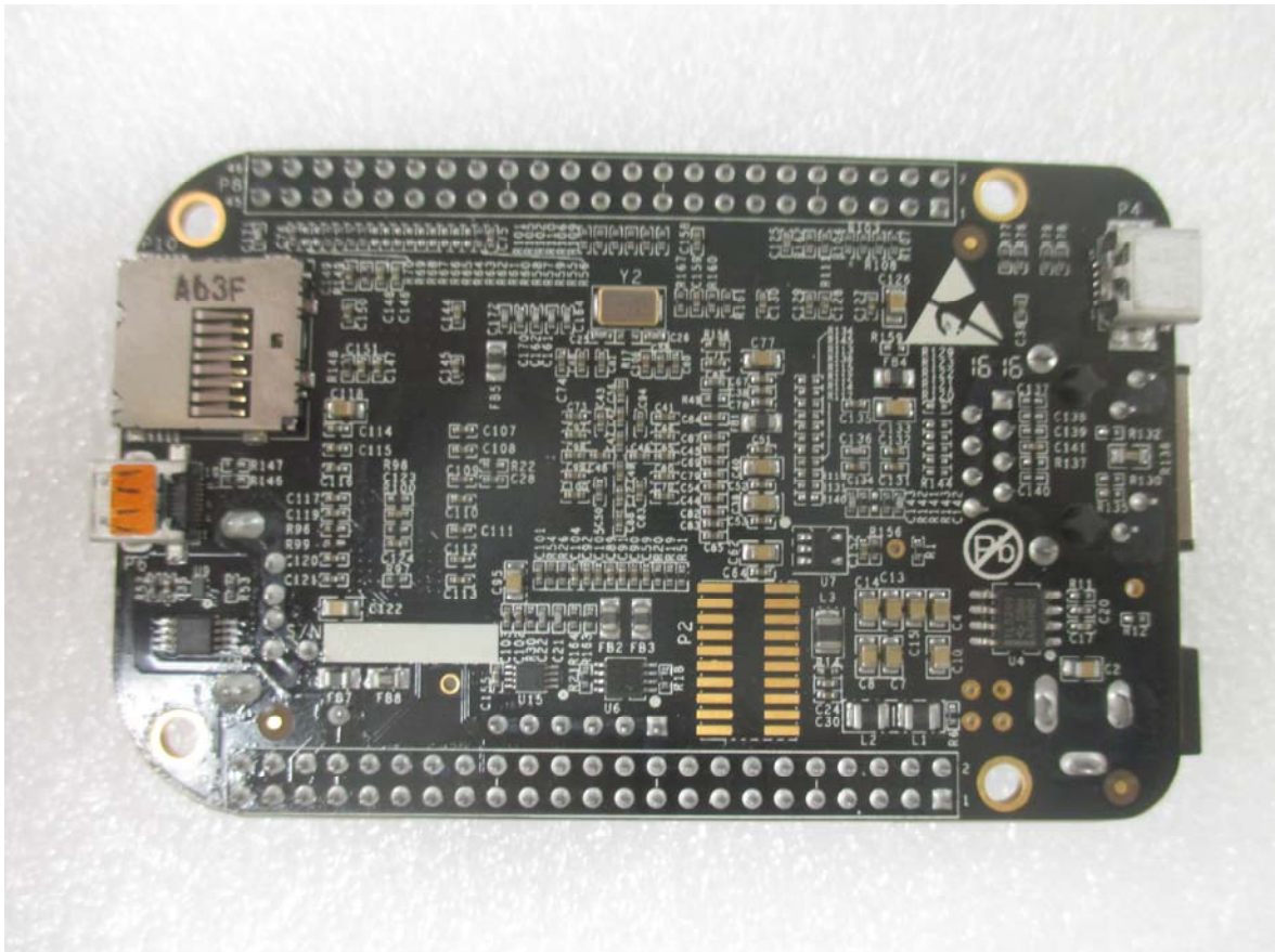
8.10 UHF Daughter Board Foil Side View
