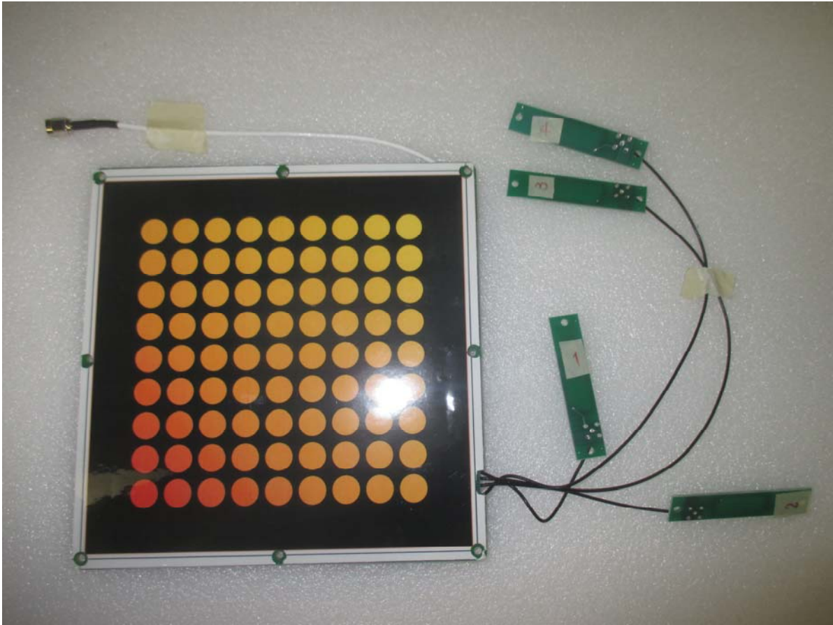
8.11 HF Board Front Side View
