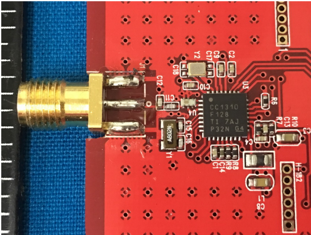
SUB 1G RF Chip IC – Top View
