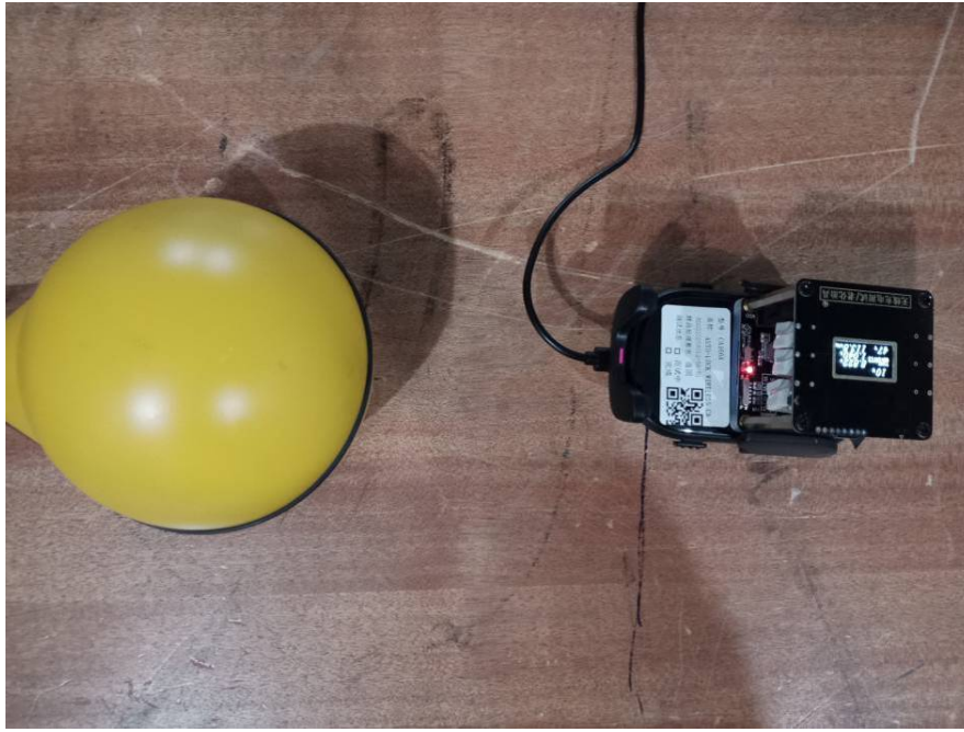
H-Filed Strength View Position A (Test distance: 15cm)
