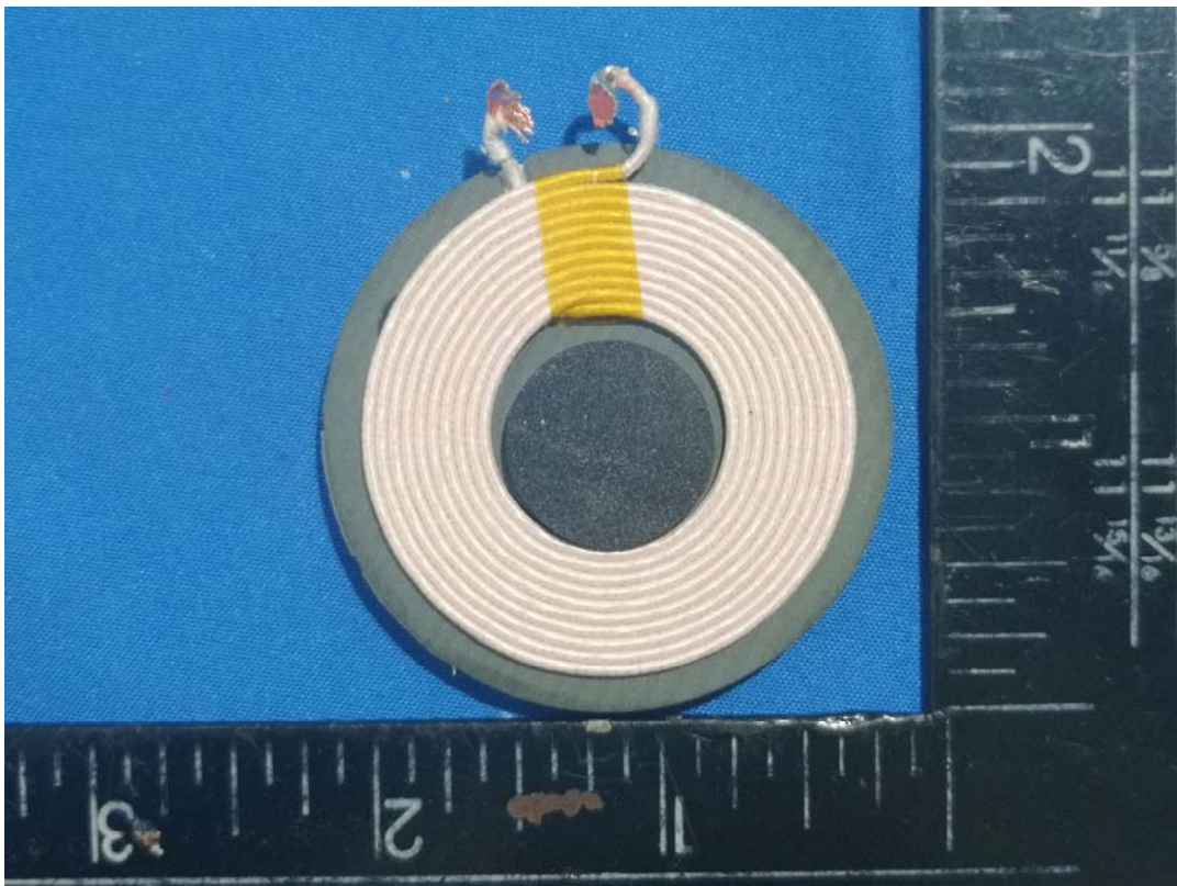
Coil Antenna
