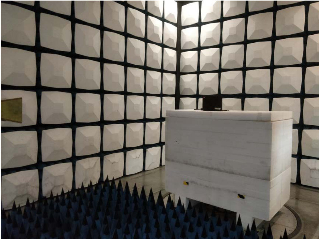
RE Above 1GHz View
