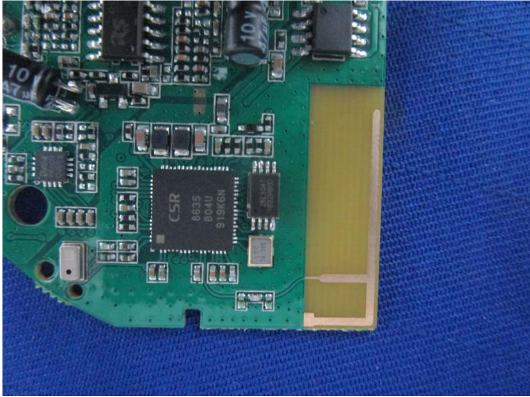
RF chip&ANT
