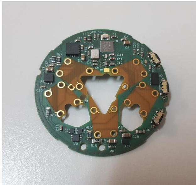
Photo 4 : PCB back side view
