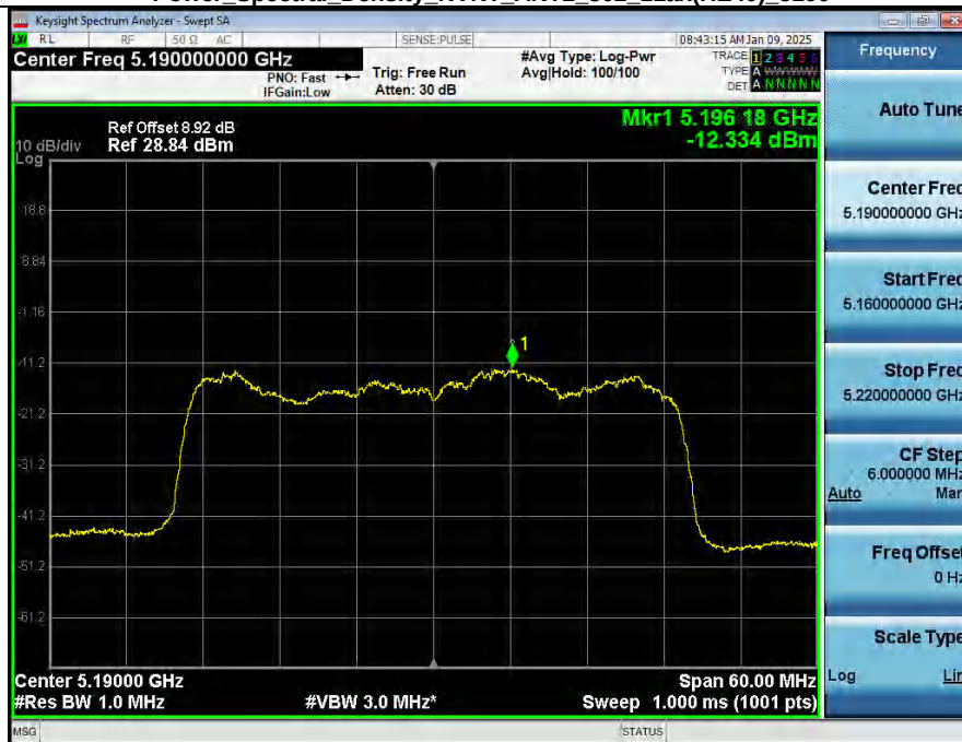
Power_Spectral_Density_NVNT_ANT2_802_11ax(HE40)_5190
