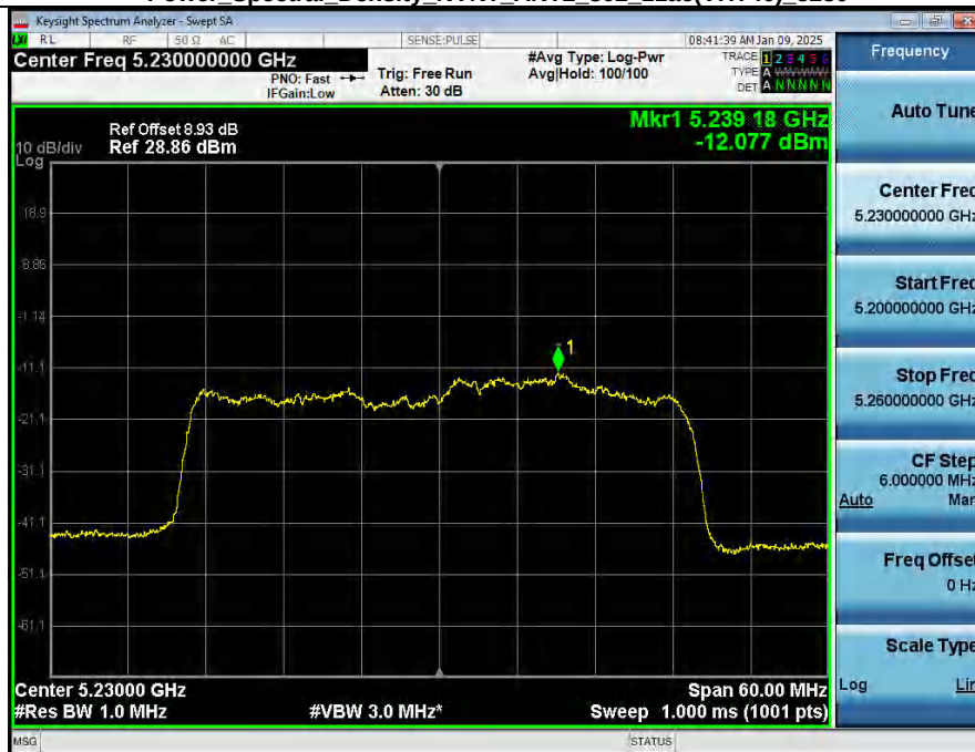
Power_Spectral_Density_NVNT_ANT2_802_11ac(VHT40)_5230
