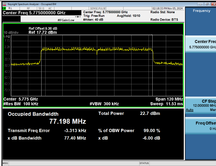
-6dB Emission Bandwidth_NVNT_ANT2_802_11ax(HE80)_5775_80M
