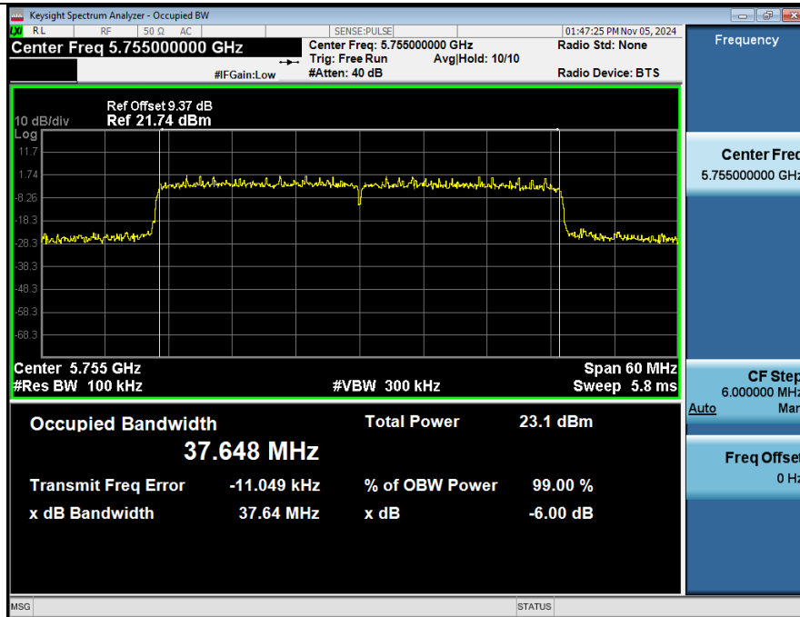
-6dB Emission Bandwidth_NVNT_ANT2_802_11ax(HE40)_5755_40M
