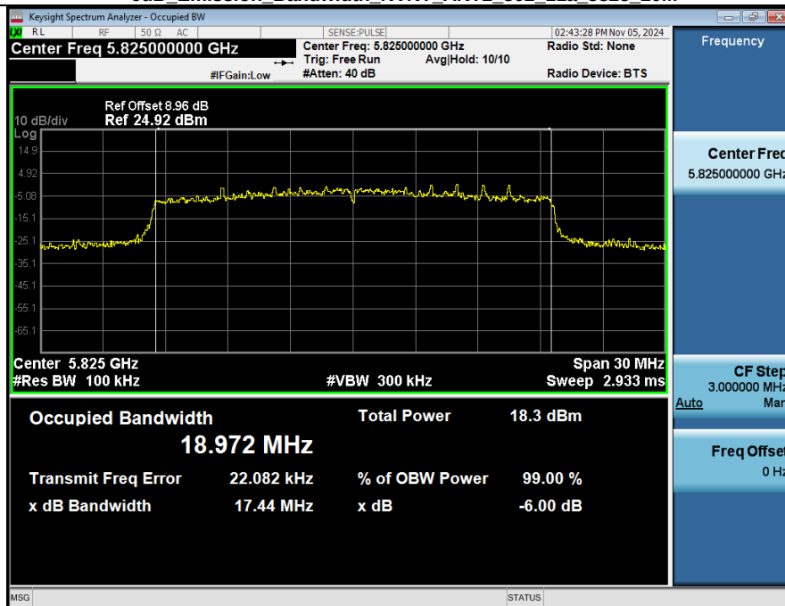
-6dB Emission Bandwidth NVNT_ANT2_802_11a_5825_20M
