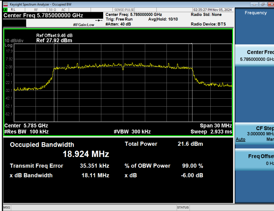
-6dB Emission Bandwidth NVNT_ANT2_802_11a_5785_20M
