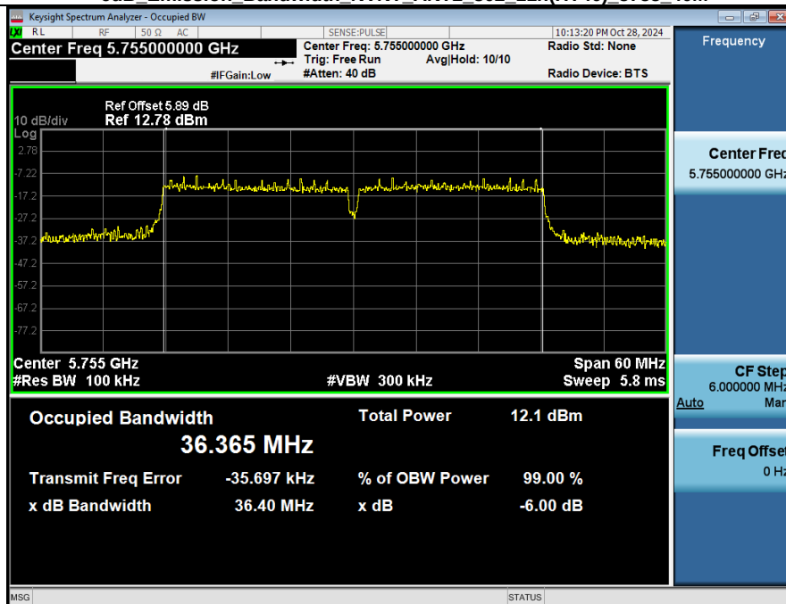
-6dB_Emission_Bandwidth_NVNT_ANT2_802_11n(HT40)_5755_40M
