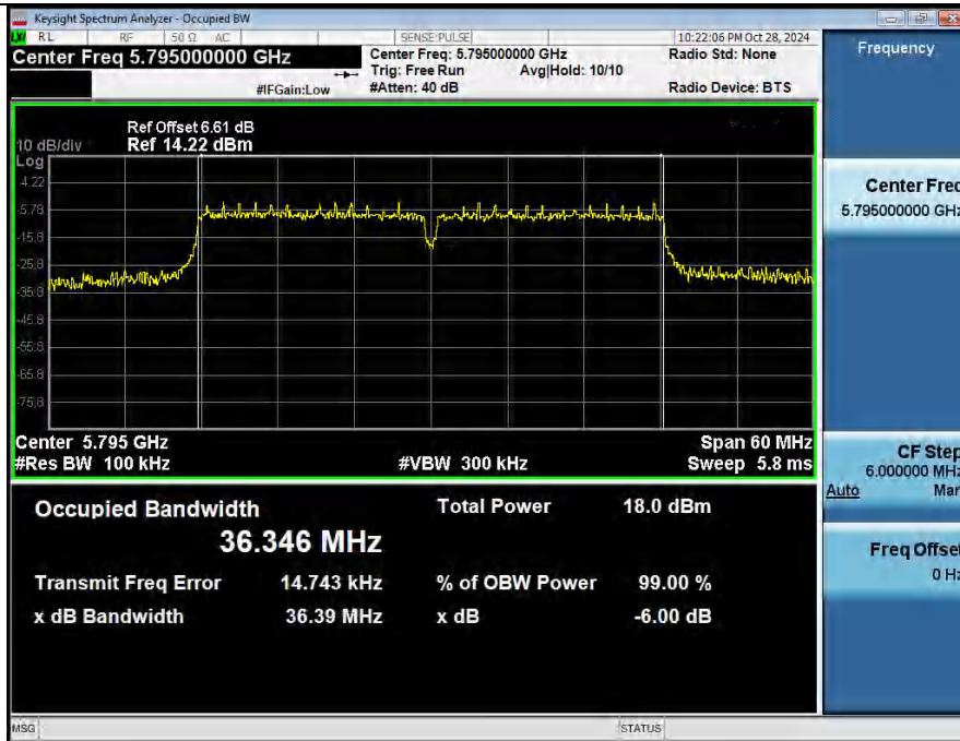
-6dB_Emission_Bandwidth_NVNT_ANT2_802_11n(HT40)_5795_40M
