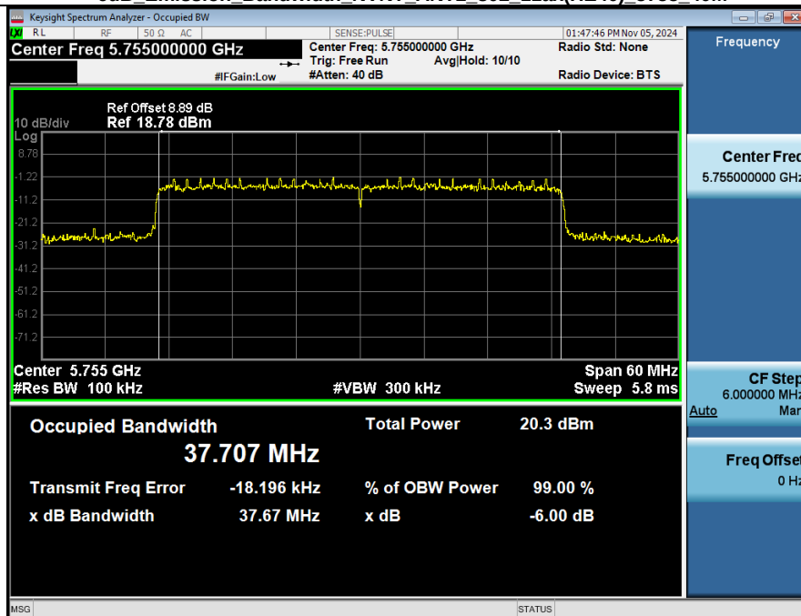
-6dB Emission Bandwidth_NVNT_ANT2_802_11ax(HE40)_5755_40M
