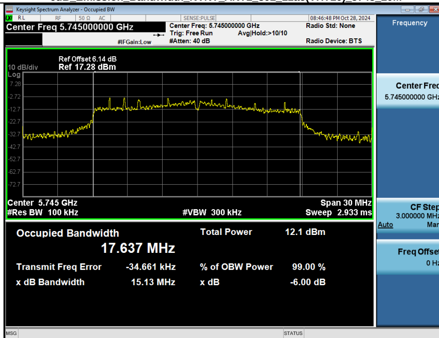
-6dB Emission Bandwidth_NVNT_ANT2_802_11ac(VHT20)_5745_20M
