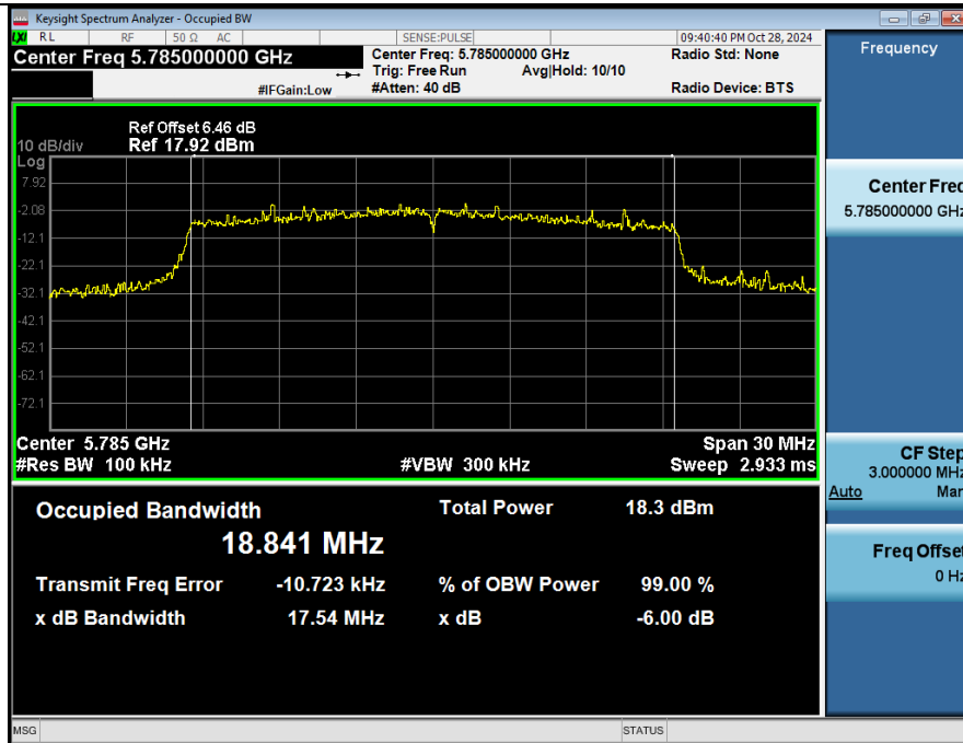
-6dB Emission Bandwidth_NVNT_ANT2_802_11ax(HE20)_5785_20M
