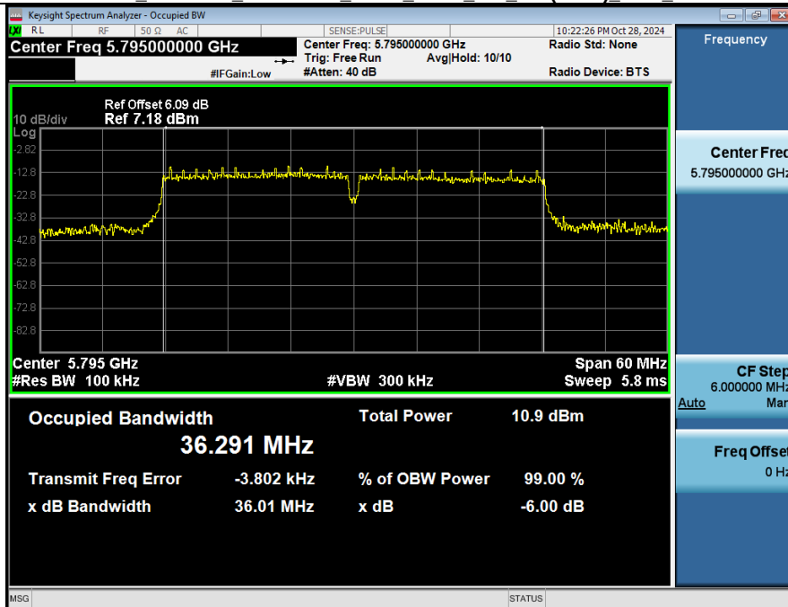
-6dB_Emission_Bandwidth_NVNT_ANT2_802_11n(HT40)_5795_40M
