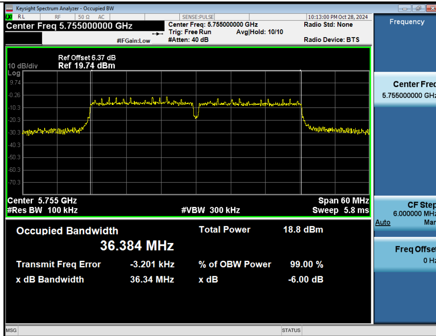
-6dB_Emission_Bandwidth_NVNT_ANT2_802_11n(HT40)_5755_40M
