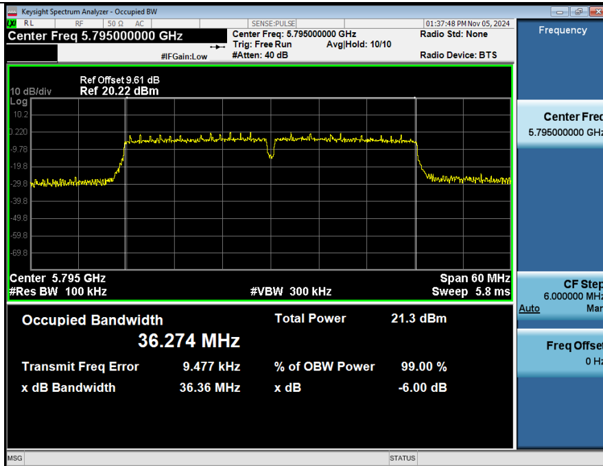
-6dB Emission Bandwidth_NVNT_ANT2_802_11ac(VHT40)_5795_40M
