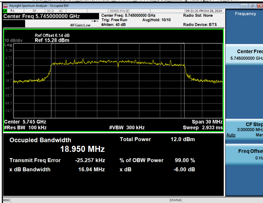
-6dB Emission Bandwidth_NVNT_ANT2_802_11ax(HE20)_5745_20M
