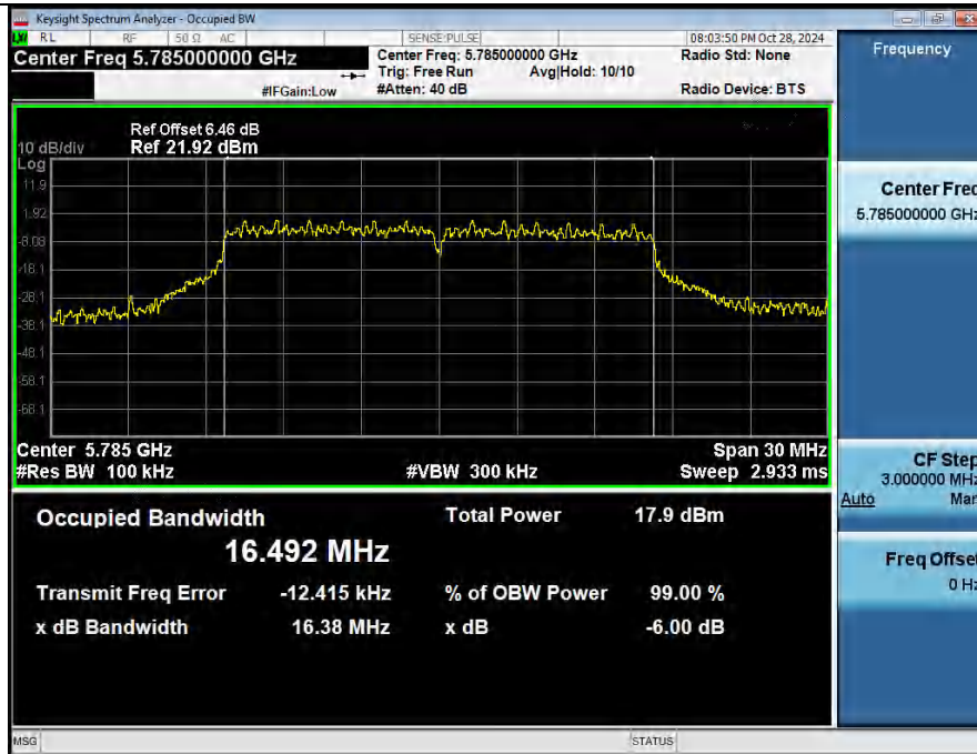
-6dB_Emission_Bandwidth_NVNT_ANT2_802_11n(HT20)_5785_20M
