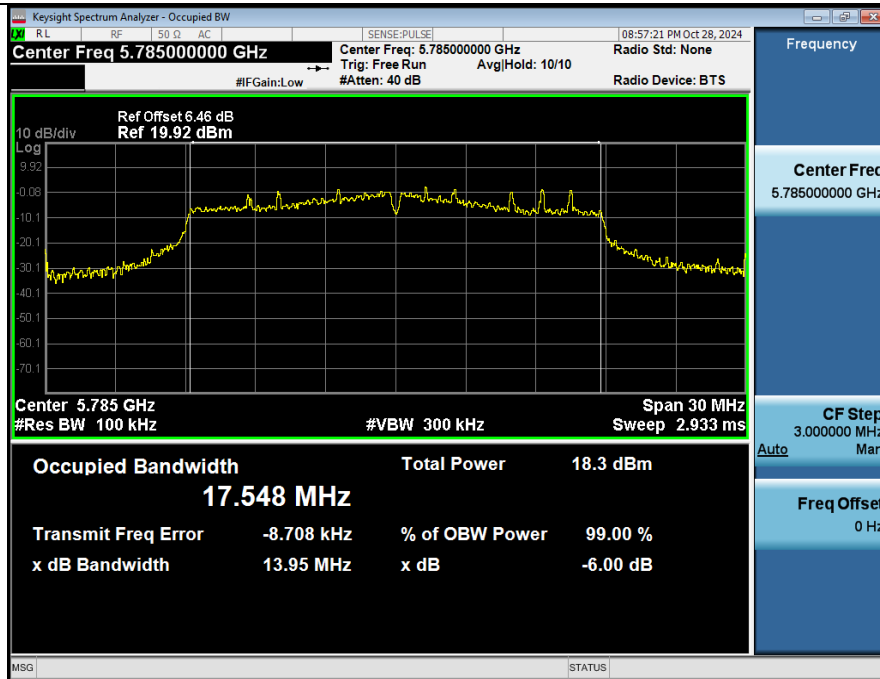
-6dB Emission Bandwidth_NVNT_ANT2_802_11ac(VHT20)_5785_20M
