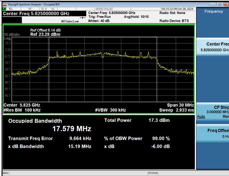
-6dB Emission Bandwidth_NVNT_ANT2_802_11ac(VHT20)_5825_20M
