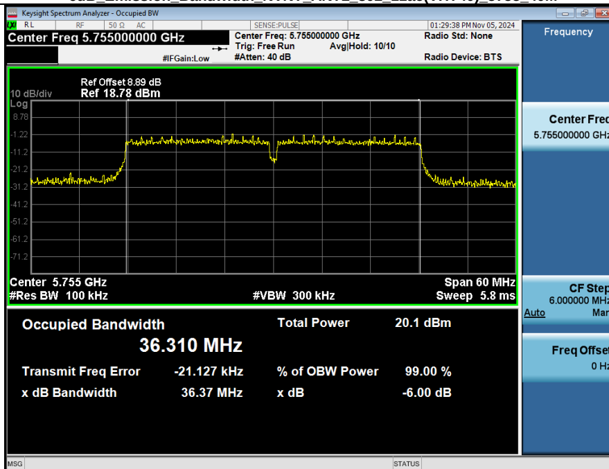
-6dB Emission Bandwidth_NVNT_ANT2_802_11ac(VHT40)_5755_40M
