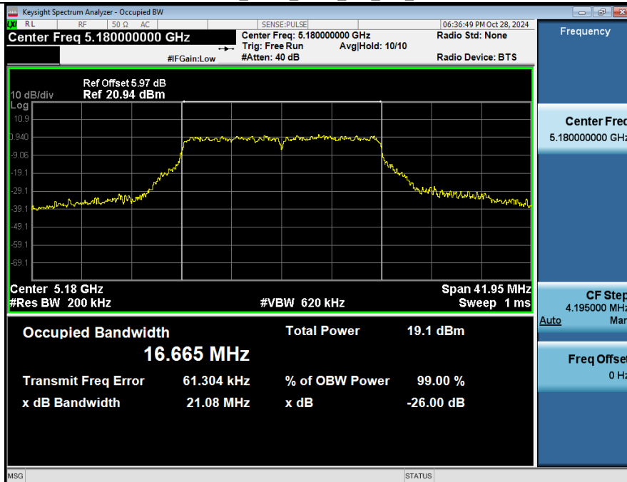
-26BW_NVNT_ANT1_802_11a_5180
