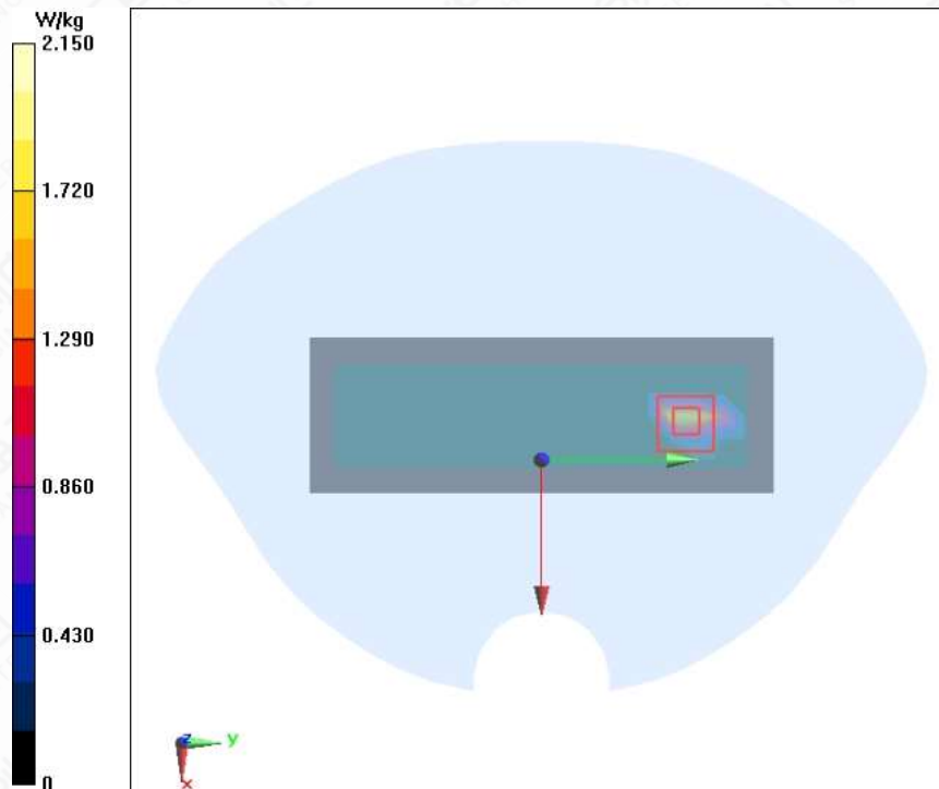
Figure A.1-10 Wi-Fi 5G U-NII-2C 11a ANT1 Left Mode Low 0mm Body
