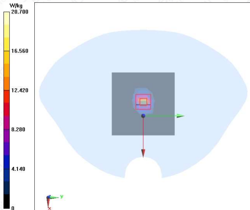
Figure A.2-7 System Check Head 5800MHz
