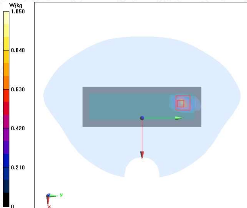
Figure A.1-11 Wi-Fi 5G U-NII-2C 11a ANT2 Right Mode Low 0mm Head
