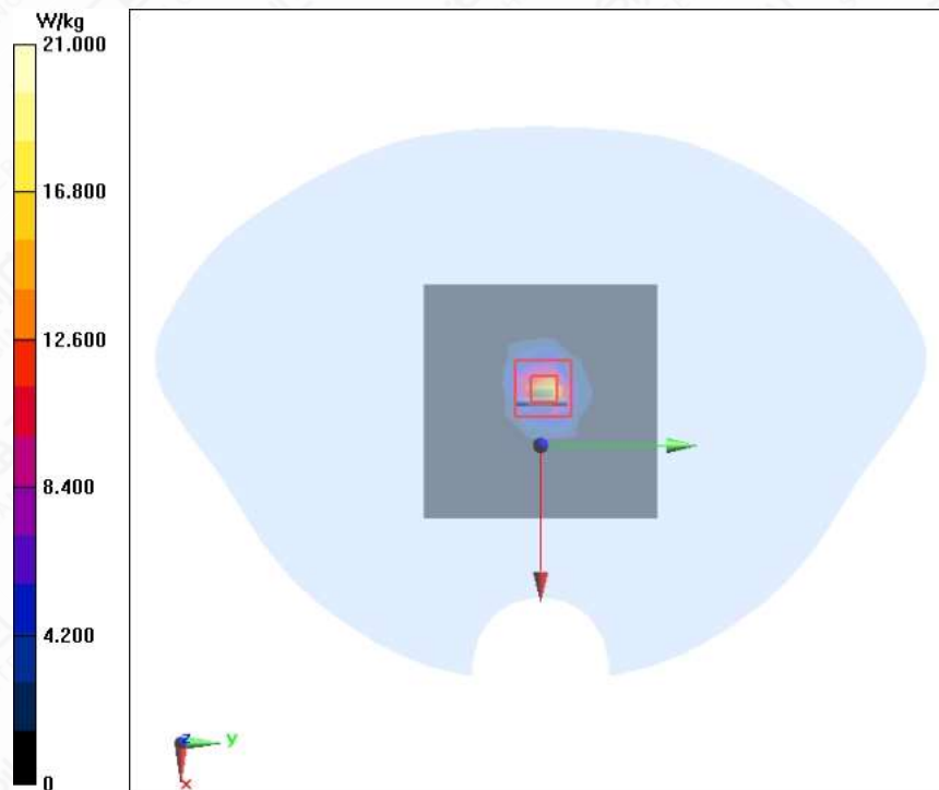
Figure A.2-6 System Check Head 5800MHz
