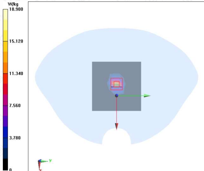
Figure A.2-1 System Check Head 5200MHz
