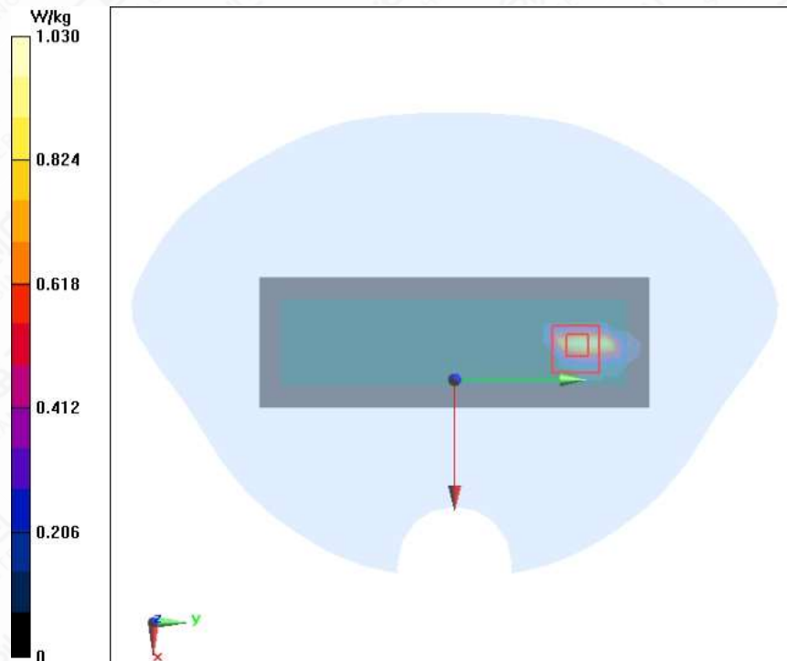
Figure A.1-13 Wi-Fi 5G U-NII-3 11a ANT1 Left Mode Low 0mm Head
