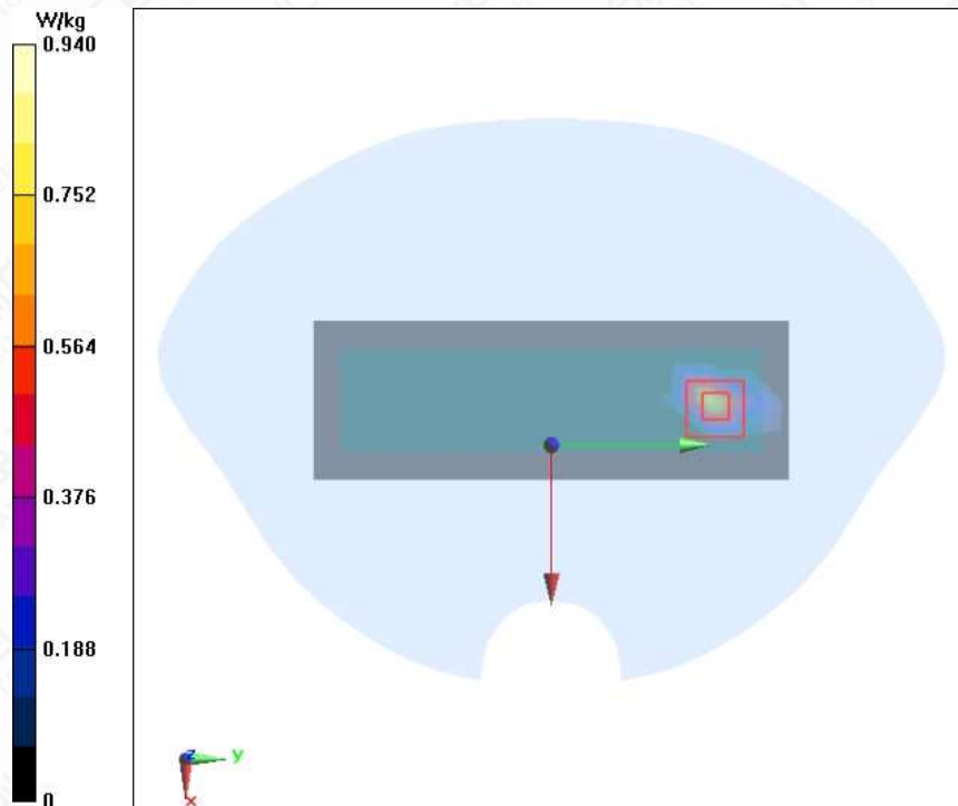
Figure A.1-9 Wi-Fi 5G U-NII-2C 11a ANT1 Left Mode Low 0mm Head
