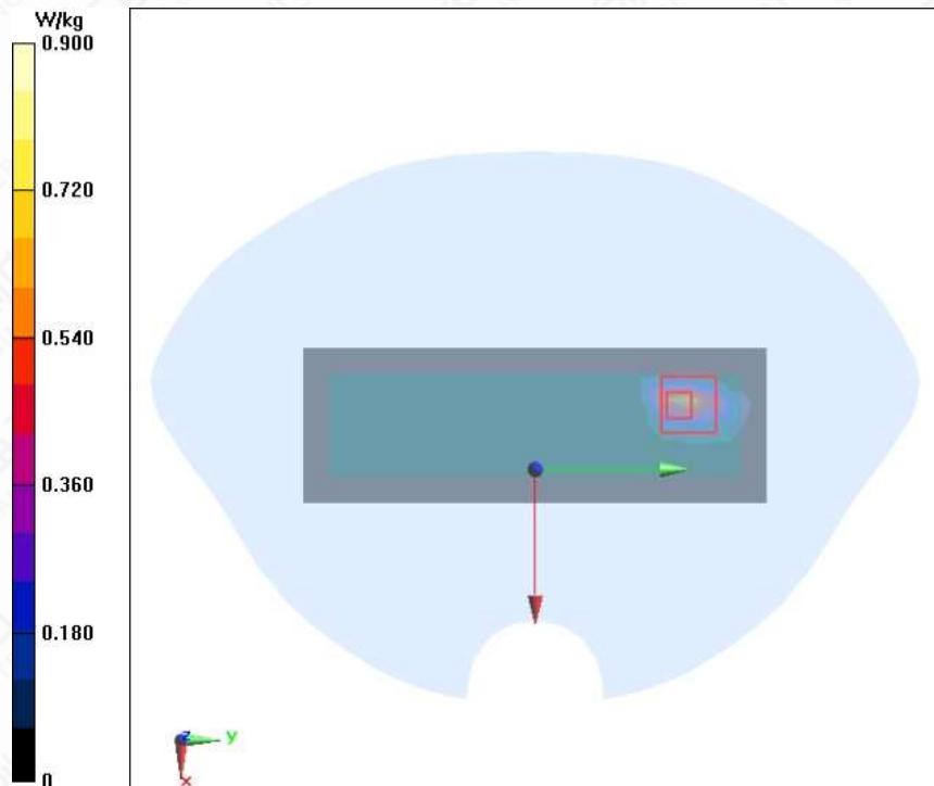
Figure A.1-7 Wi-Fi 5G U-NII-2A 11a ANT2 Right Mode Low 0mm Head
