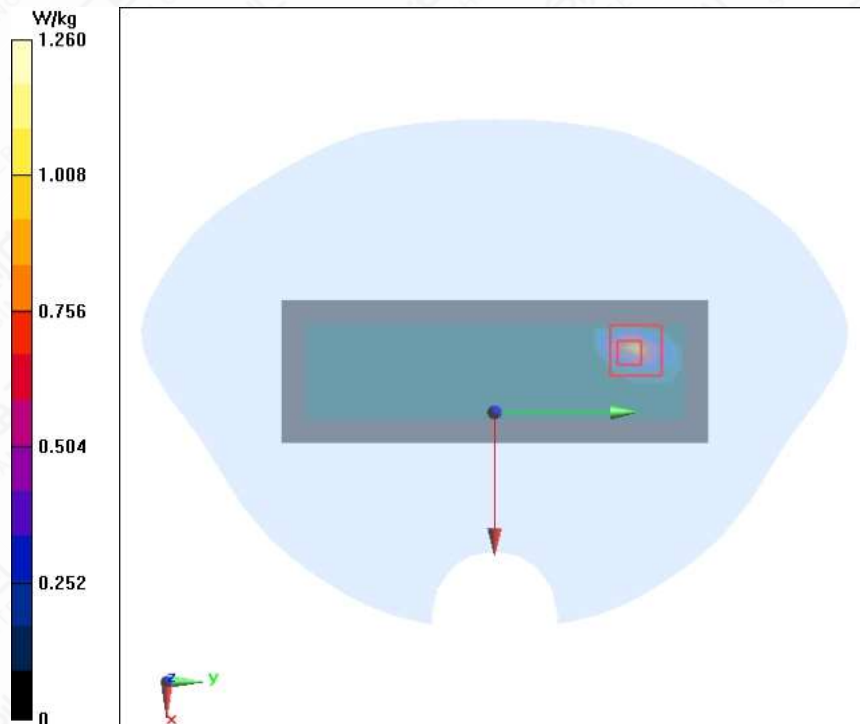
Figure A.1-8 Wi-Fi 5G U-NII-2A 11a ANT2 Right Mode Low 0mm Body
