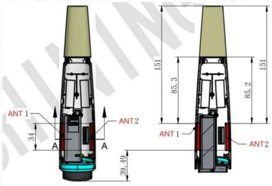
Figure 12.2-1 Antenna Locations(Front View)
