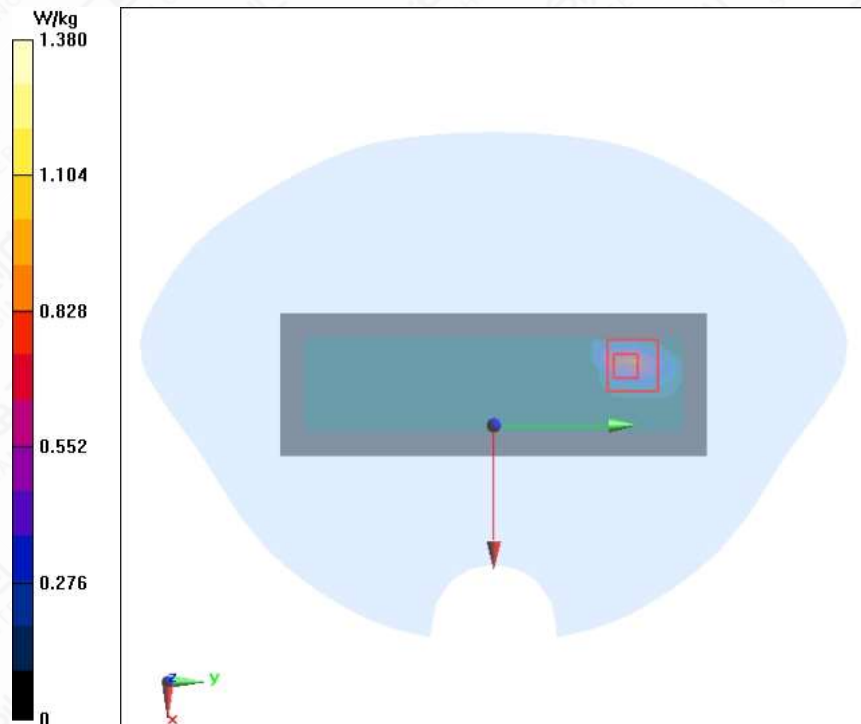
Figure A.1-4 Wi-Fi 5G U-NII-1 11a ANT2 Right Mode Low 0mm Body
