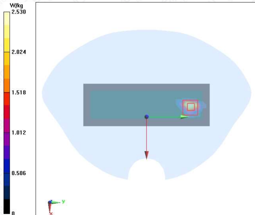
Figure A.1-14 Wi-Fi 5G U-NII-3 11a ANT1 Left Mode Low 0mm Body
