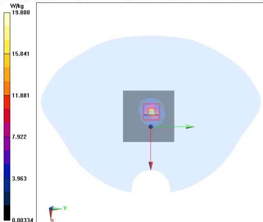
Figure A.2-2 System Check Head 5300MHz
