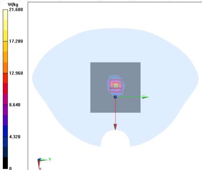
Figure A.2-4 System Check Head 5600MHz
