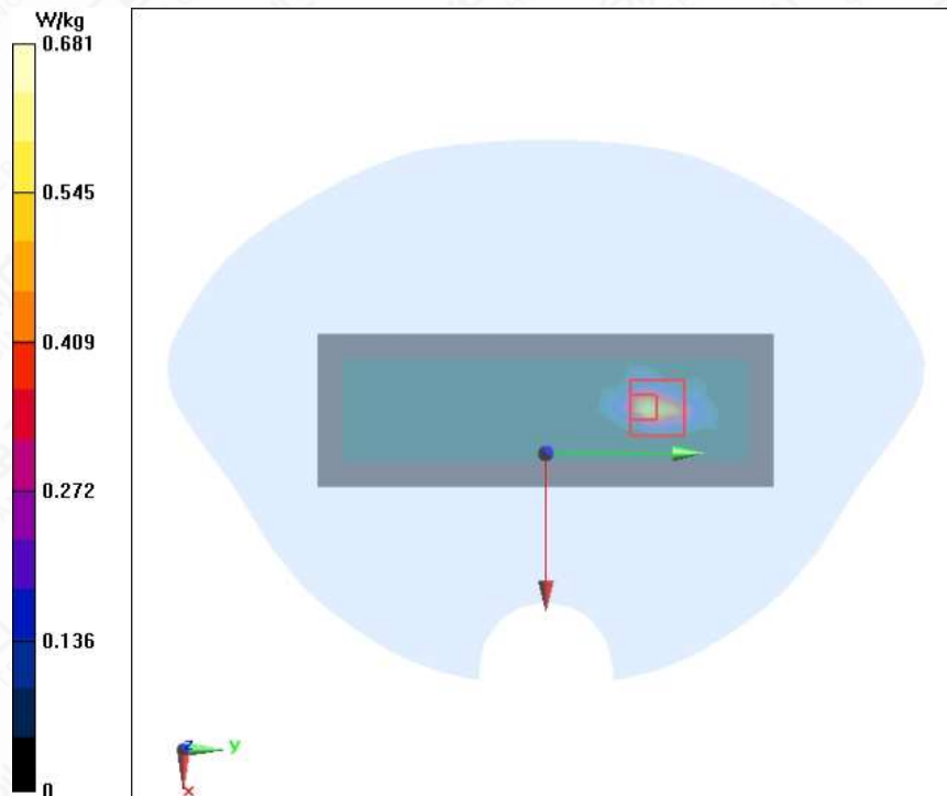
Figure A.1-15 Wi-Fi 5G U-NII-3 11a ANT2 Right Mode High 0mm Head
