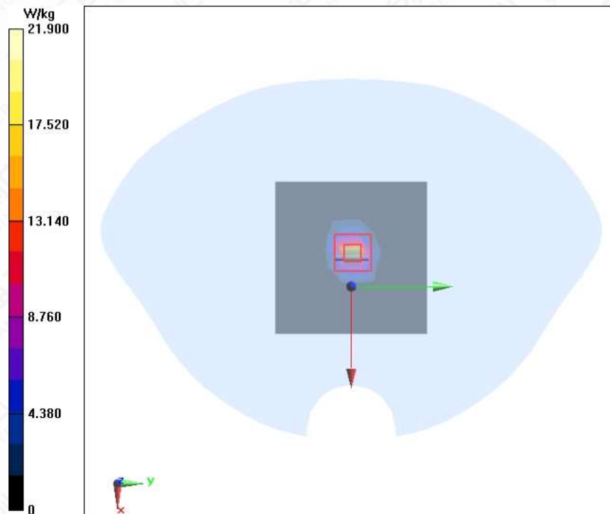
Figure A.2-5 System Check Head 5600MHz
