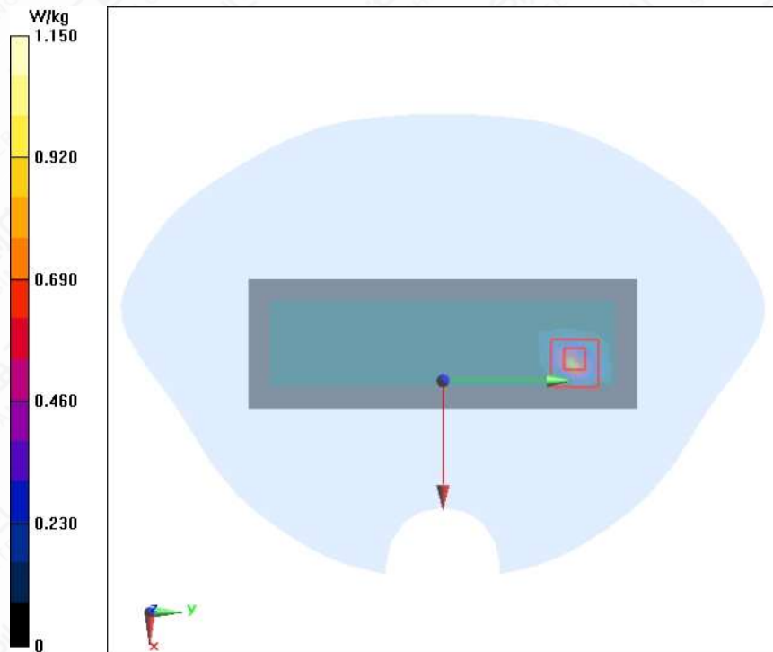
Figure A.1-2 Wi-Fi 5G U-NII-1 11a ANT1 Left Mode Low 0mm Body
