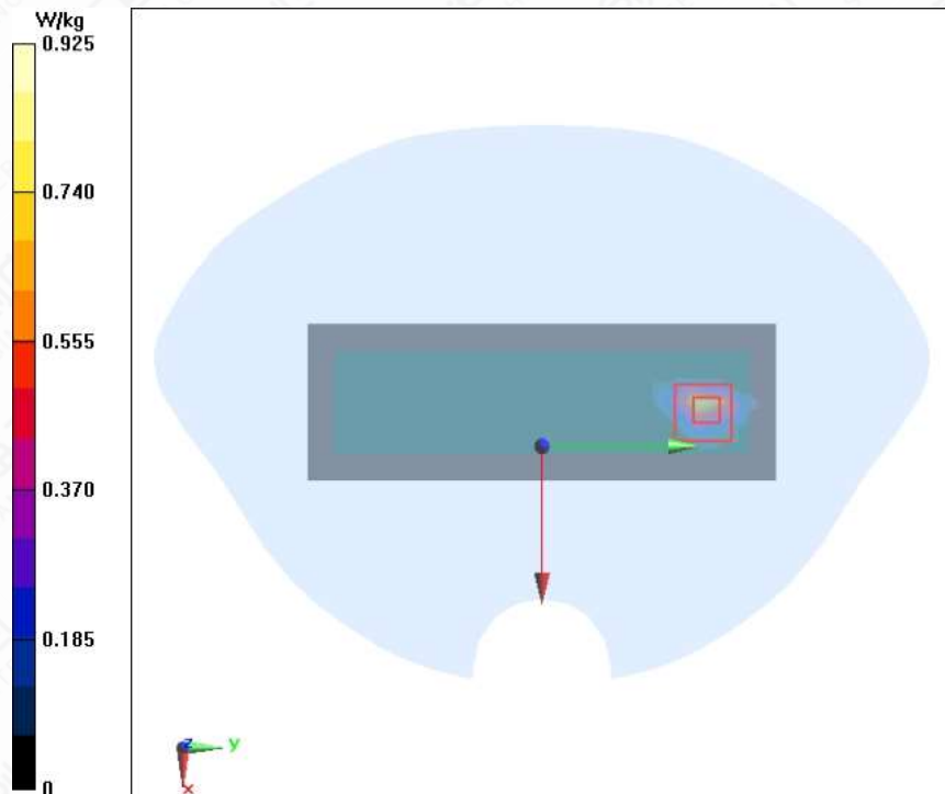
Figure A.1-6 Wi-Fi 5G U-NII-2A 11a ANT1 Left Mode Middle 0mm Body
