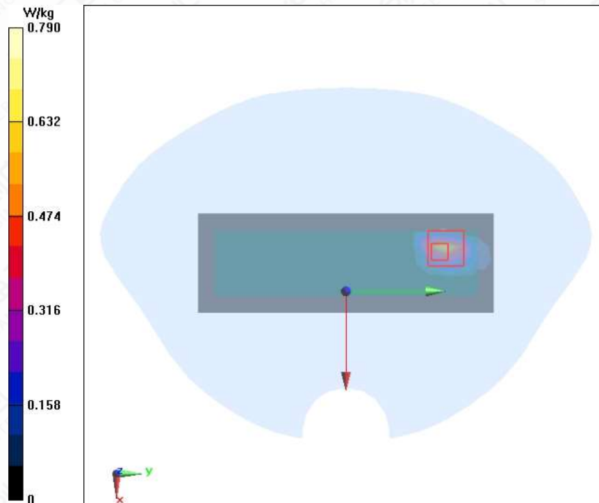
Figure A.1-3 Wi-Fi 5G U-NII-1 11a ANT2 Right Mode Low 0mm Head
