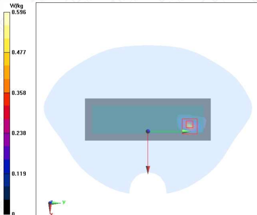
Figure A.1-1 Wi-Fi 5G U-NII-1 11a ANT1 Left Mode Low 0mm Head
