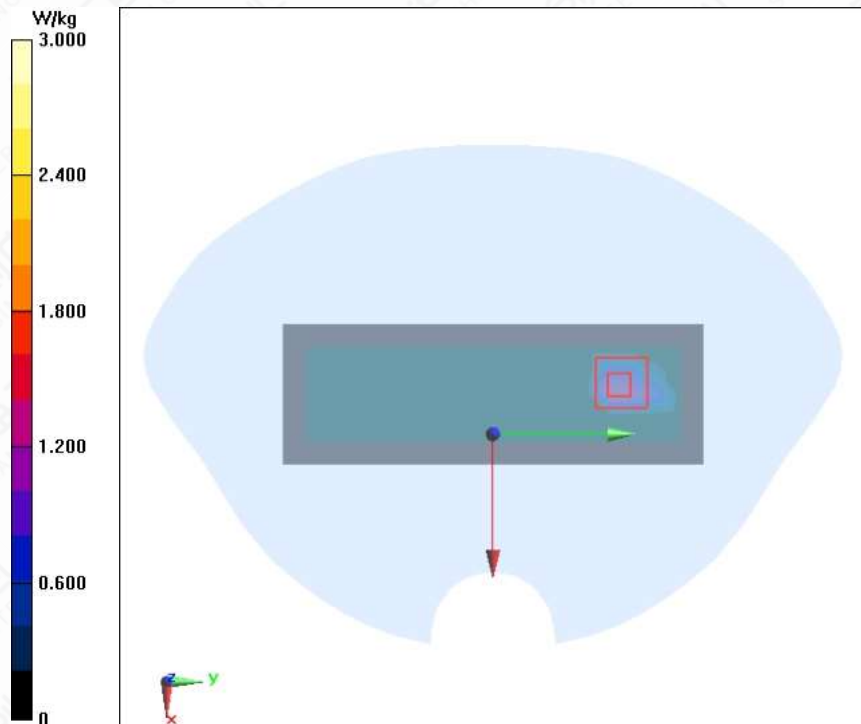
Figure A.1-12 Wi-Fi 5G U-NII-2C 11a ANT2 Right Mode Low 0mm Body
