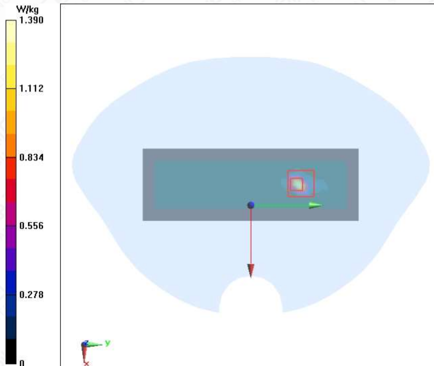
Figure A.1-16 Wi-Fi 5G U-NII-3 11a ANT2 Right Mode Low 0mm Body
