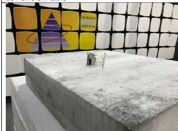
Nano: horizontal orientation: > 1 GHz; close-up EUT on 1.5m table. Absorber on floor between antenna and EUT
