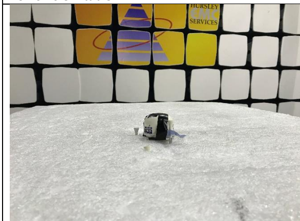
Nano: vertical orientation: 30-1000 MHz; close-up EUT on 0.8m table
