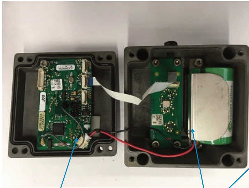
Radio card as for FM3N-VW41
