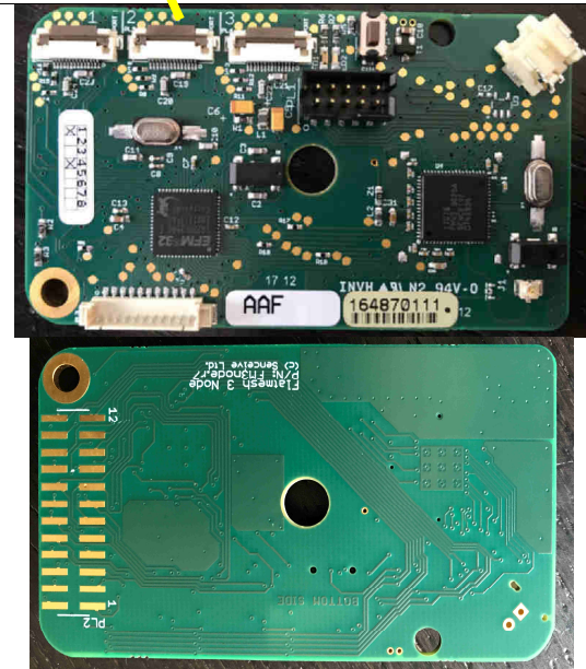
Radio PCB under side
