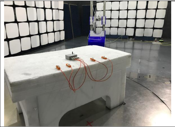
Node + cables: 30-1000 MHz; EUT on 0.8m table
