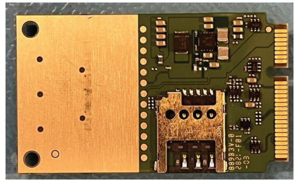
PLS62-W cellular modem
