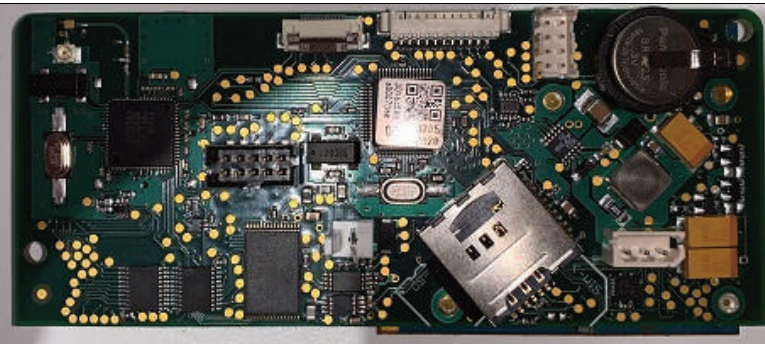
Top-side of main PCB
