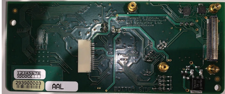
Underside of main PCB – shown with and without LTE module
