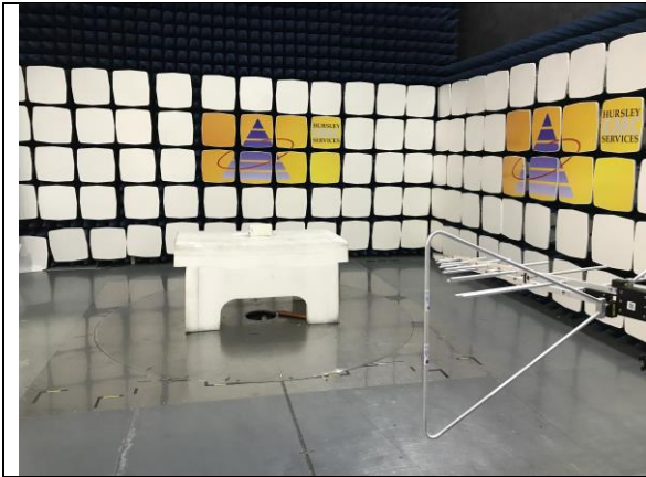
Gateway: 30-1000 MHz; EUT on 0.8m table
