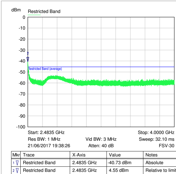
Ch 25: trace 3; 2483.5 – 4000 MHz (Peak)
