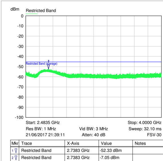
Ch 18: trace 3; 2483.5 – 4000 MHz (Peak)
