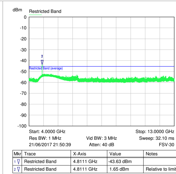
Ch 11: trace 4; 4000 – 13000 MHz (Peak)
