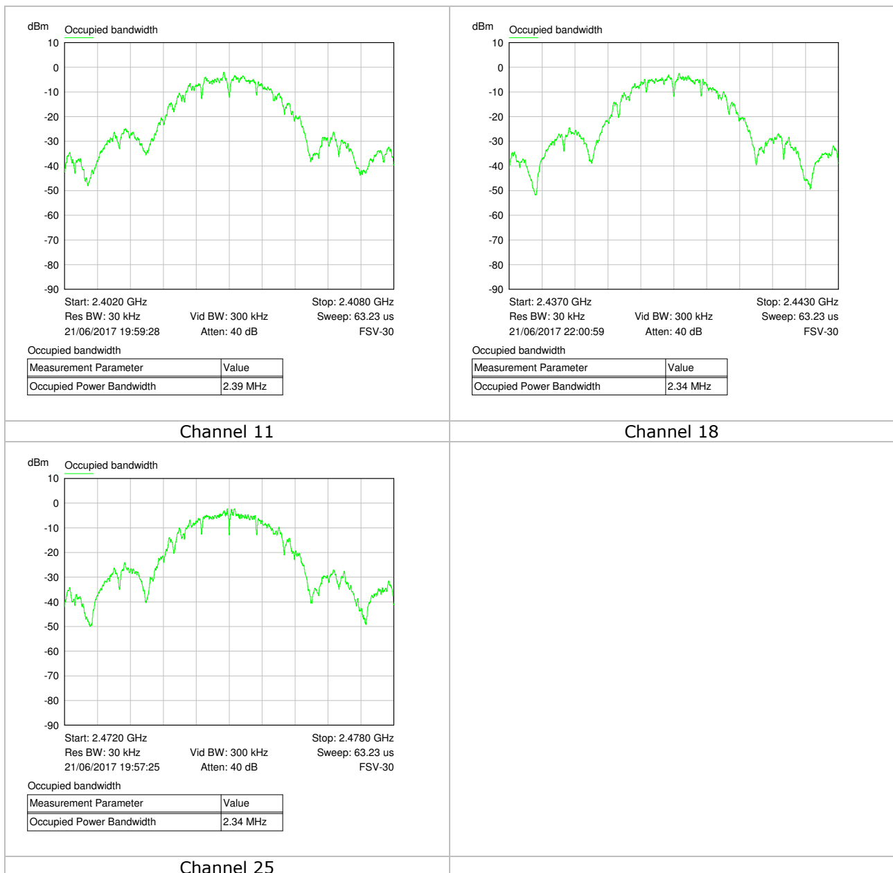
Figure 9: Occupied Bandwidth
