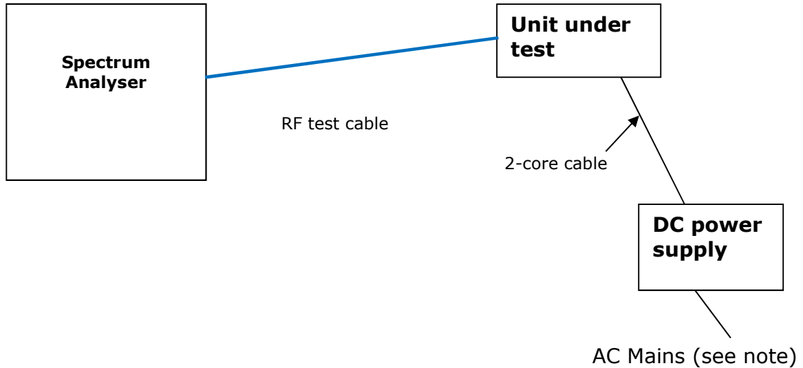
Figure 1: Test Configuration
