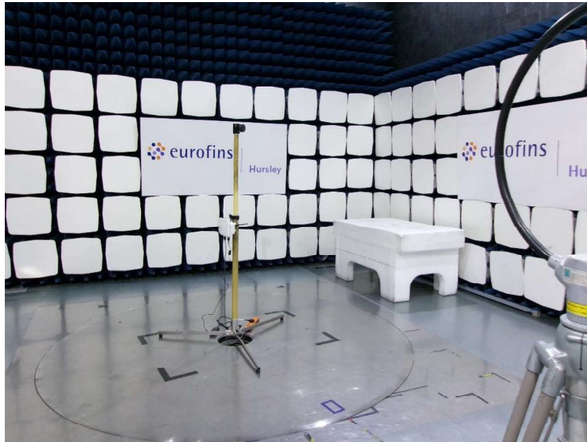
Radiated H-Field Emissions (9 kHz to 30 MHz)
