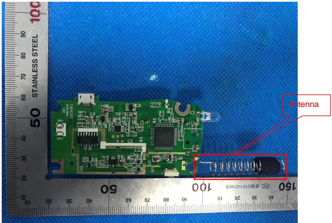
INTERNAL VIEW-2 OF EUT
