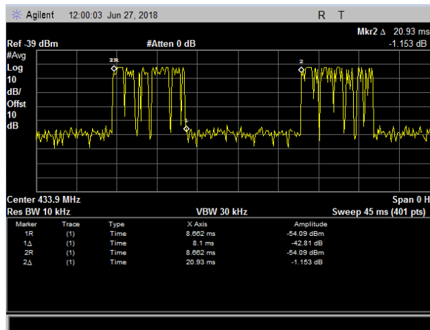
Plot 7. Field Strength of Fundamental, Duty Cycle
