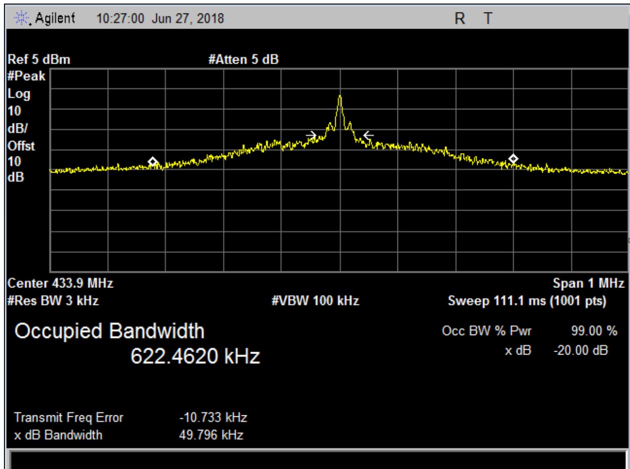
Plot 8. 20 dB Bandwidth, 433.92 MHz
