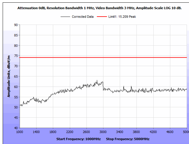
Plot 4. Field Strength of Spurious Emissions, Harmonics, 1 - 5 GHz, 15.209 Peak Limit
