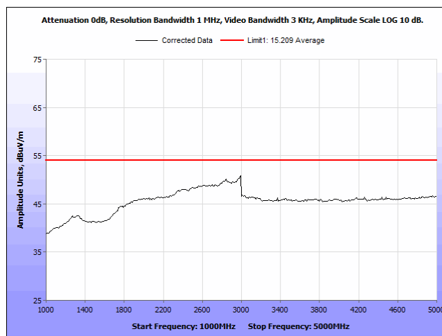
Plot 5. Field Strength of Spurious Emissions, Harmonics, 1 - 5 GHz, 15.209 Average Limit
