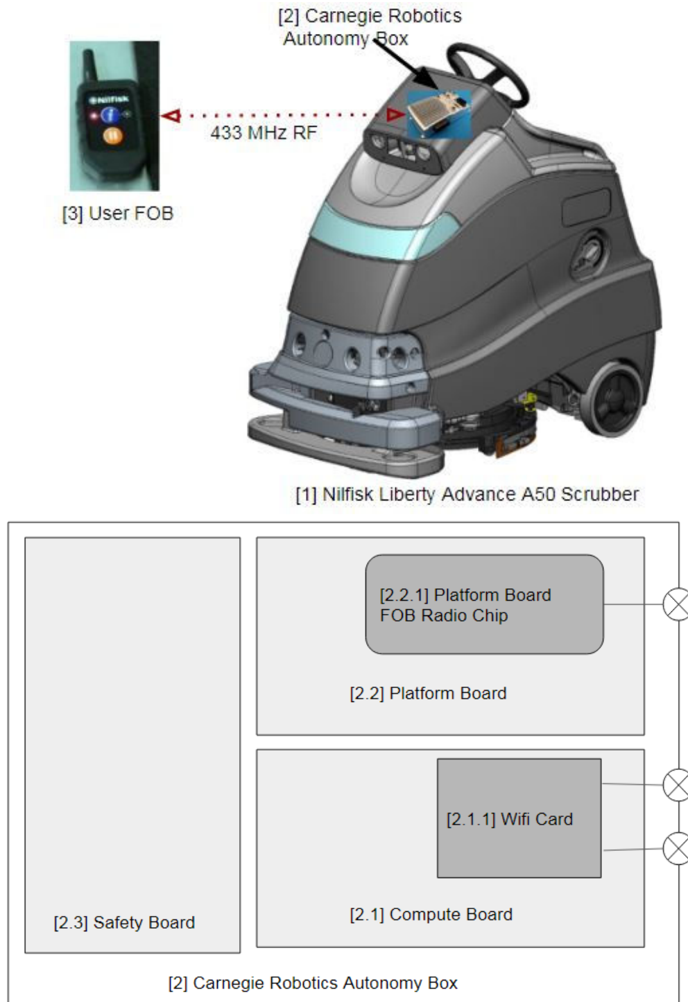
Figure 1. Block Diagram of Test Configuration
