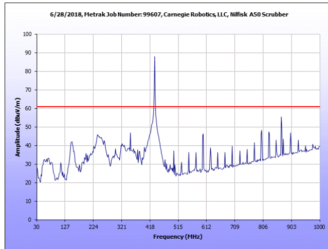
Plot 3. Field Strength of Spurious Emissions, Harmonics, 30 – 1000 MHz, 15.231 Spurious Emissions Limit
