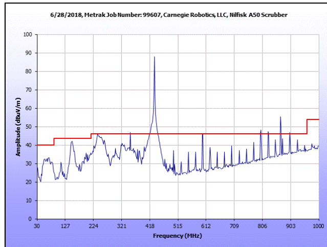
Plot 2. Field Strength of Spurious Emissions, Harmonics, 30 – 1000 MHz, 15.209 Limit
