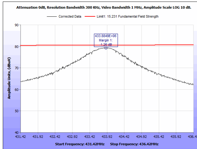
Plot 6. Field Strength of Fundamental, DCCF applied, 3m
