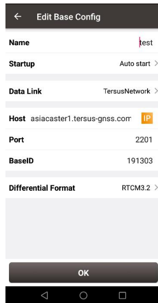
Figure 2.8 Base configuration
