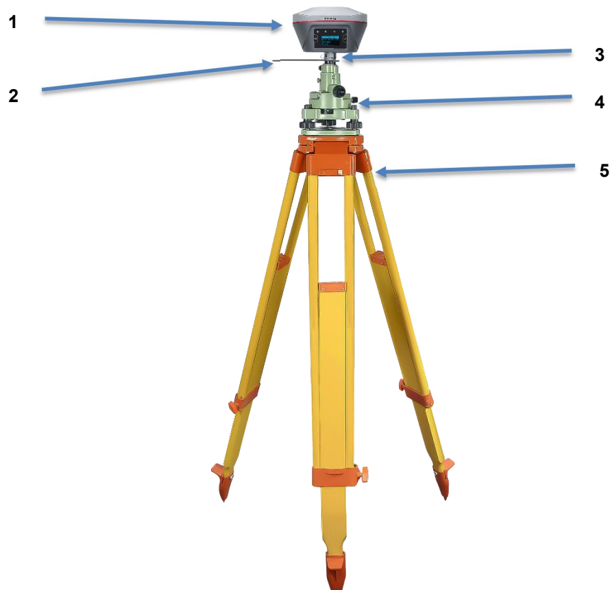
Figure 2.4 Oscar as a base without radio antenna
