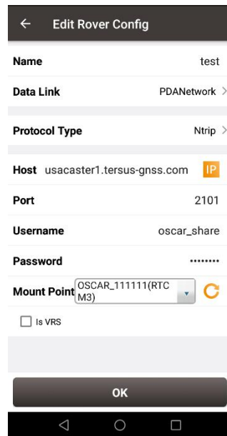
Figure 4.13 Rover configuration – PDANetwork
