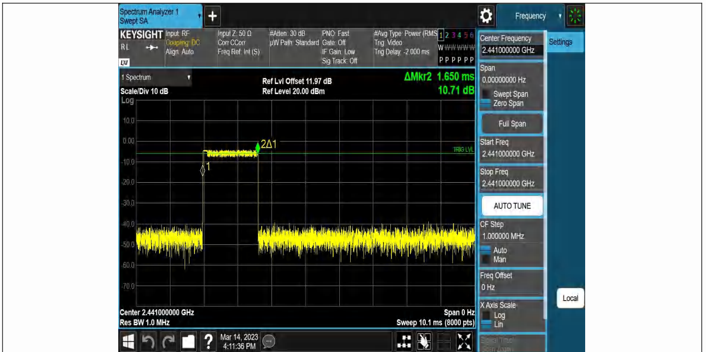
2DH3-Ant1-Hop-1.650-160
