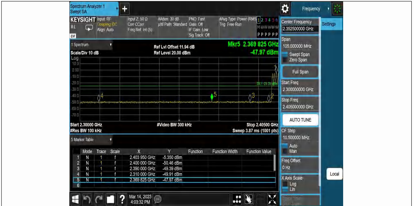
DH5-Ant1-Low-Hop_2402--5.35
