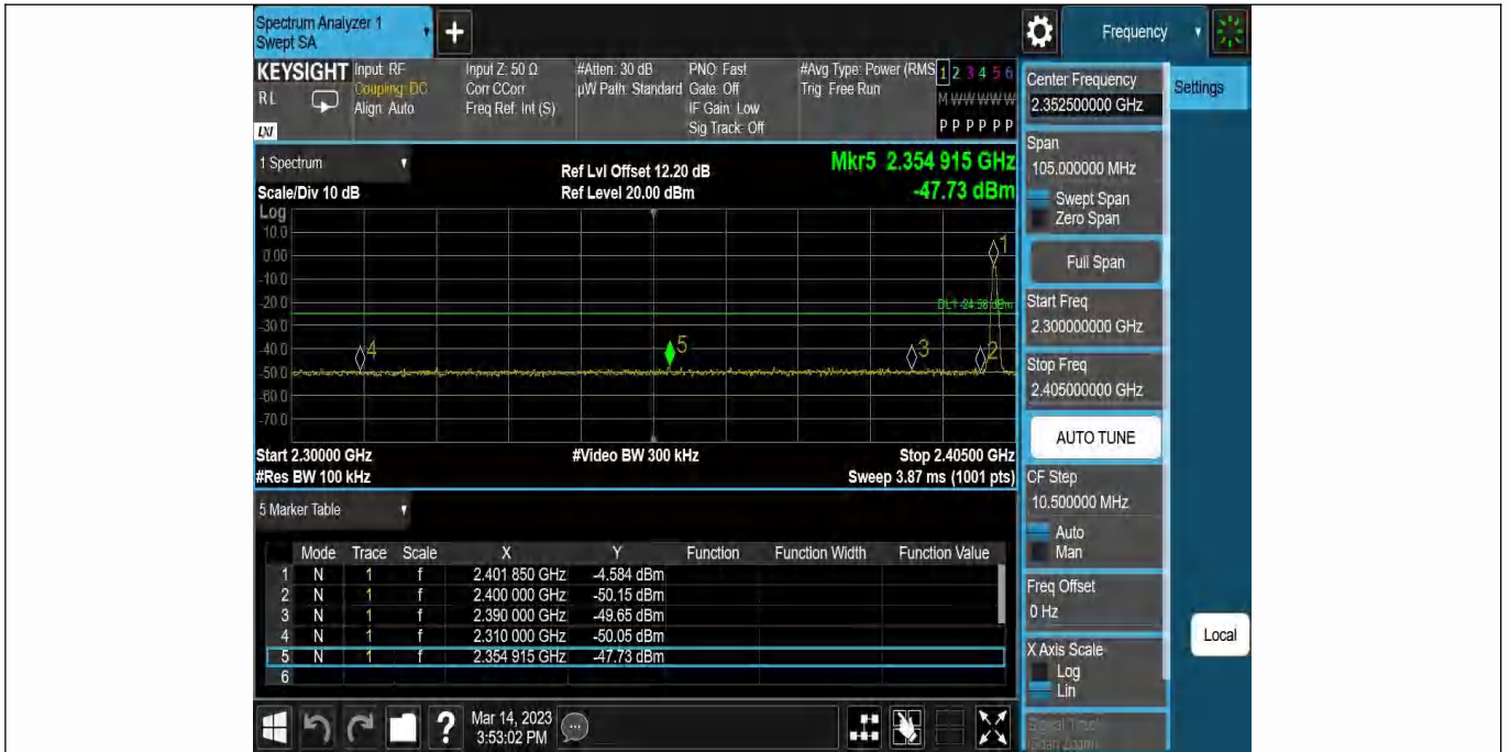
DH5-Ant1-Low-2402--4.58
