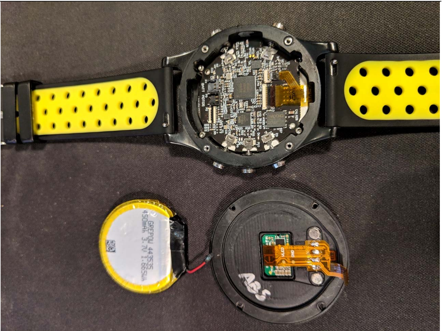
Disassembly Overview
